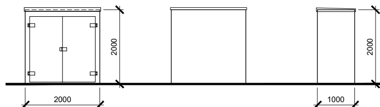
Front Elevation
