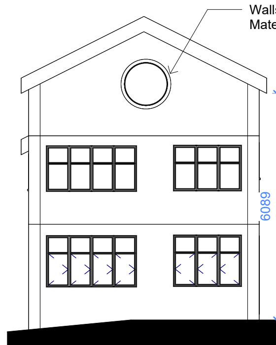
North Front -Proposed 1 : 100
