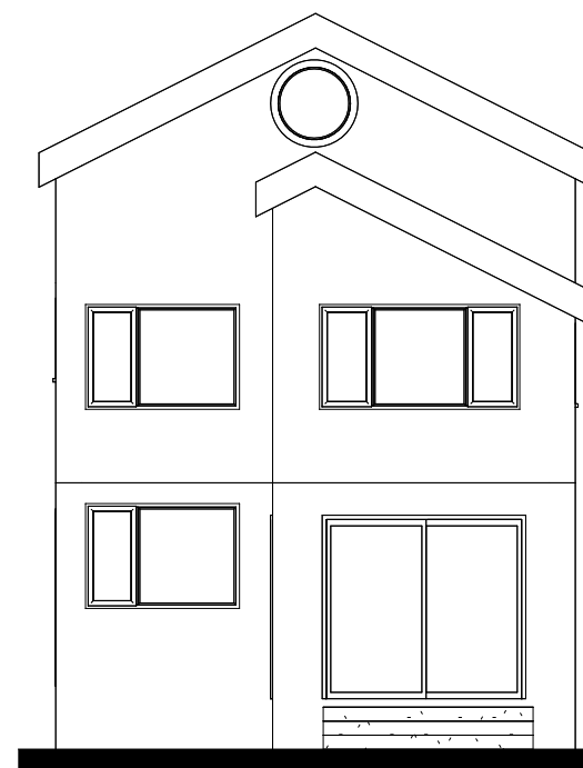
North Front -Proposed 1 : 100
