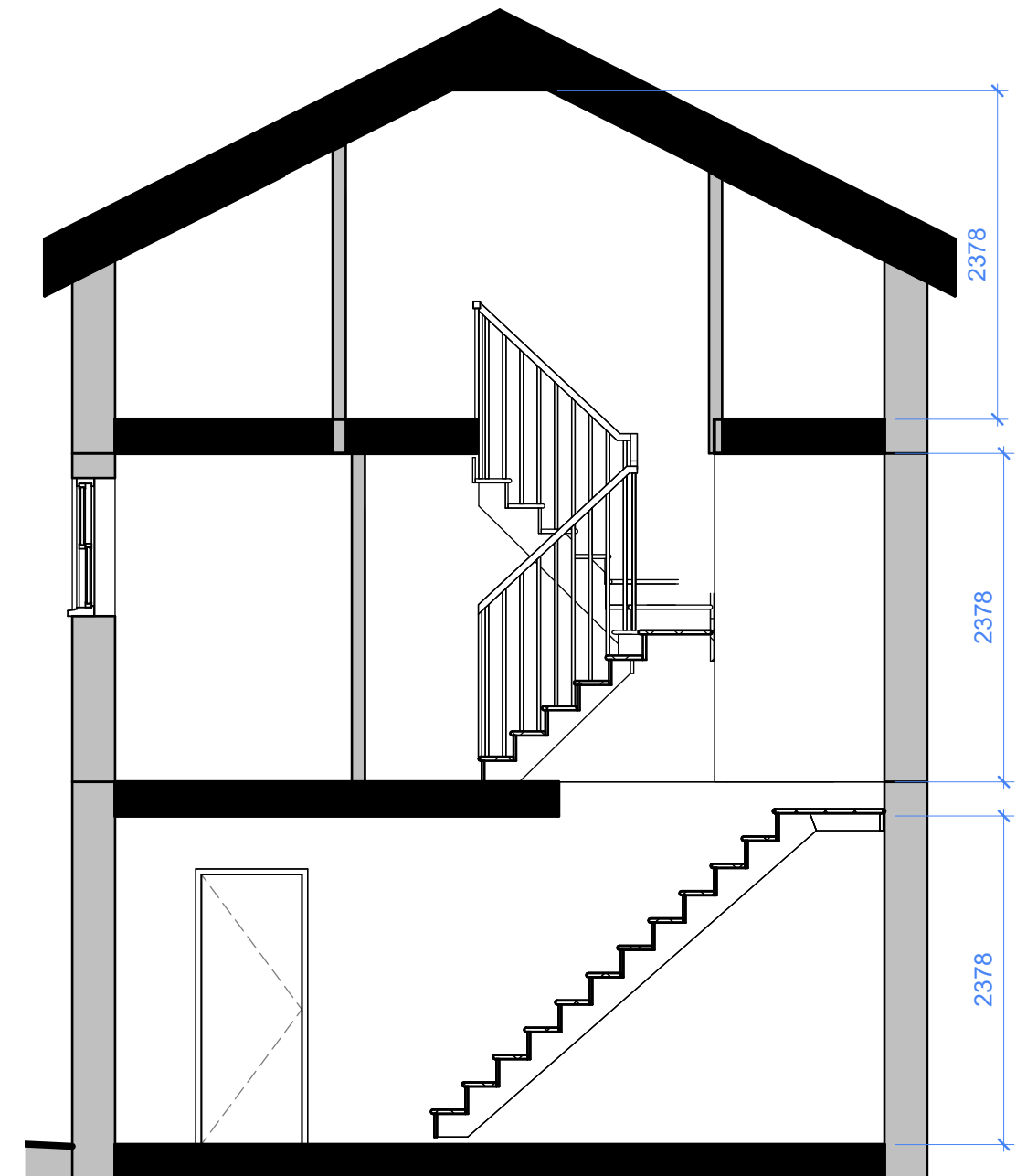
Proposed Section 1 : 50
