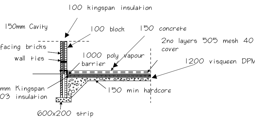
FOUNDATION DETAIL
