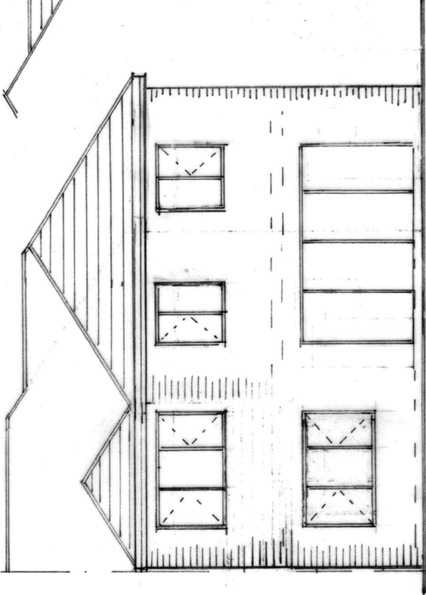
REAR ELEVATION (PROPOSED)
