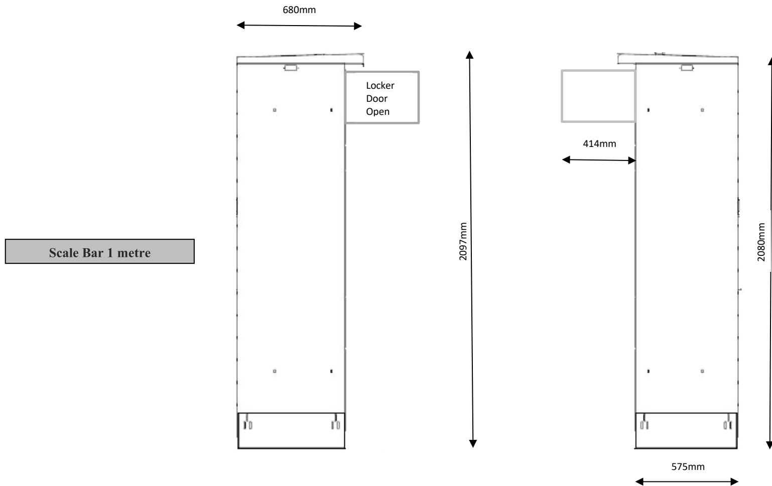
Left and Right Side Elevations Amazon Locker, Littleborough Rail Station, Station Road, Littleborough, Greater Manchester, OL15 8AF Scale 1: 20
