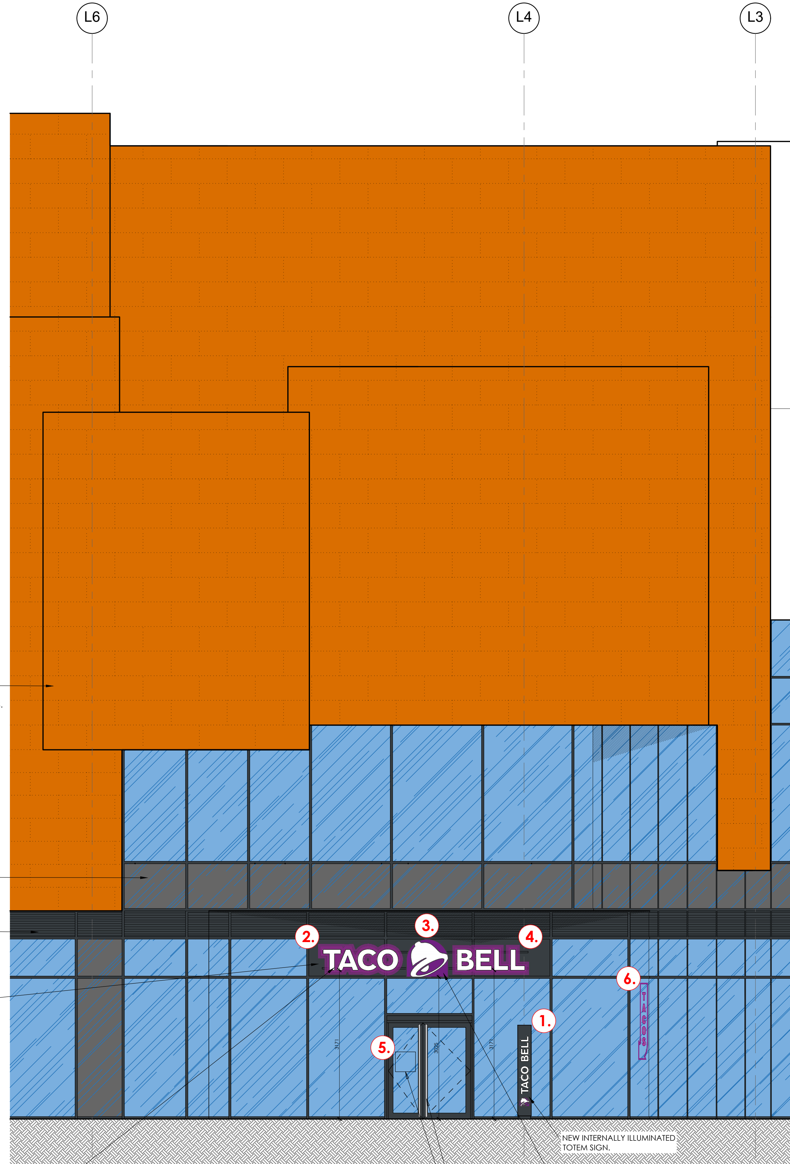
proposed North facing elevation scale - 1:50 @ A1 / 1:100 @ A3
