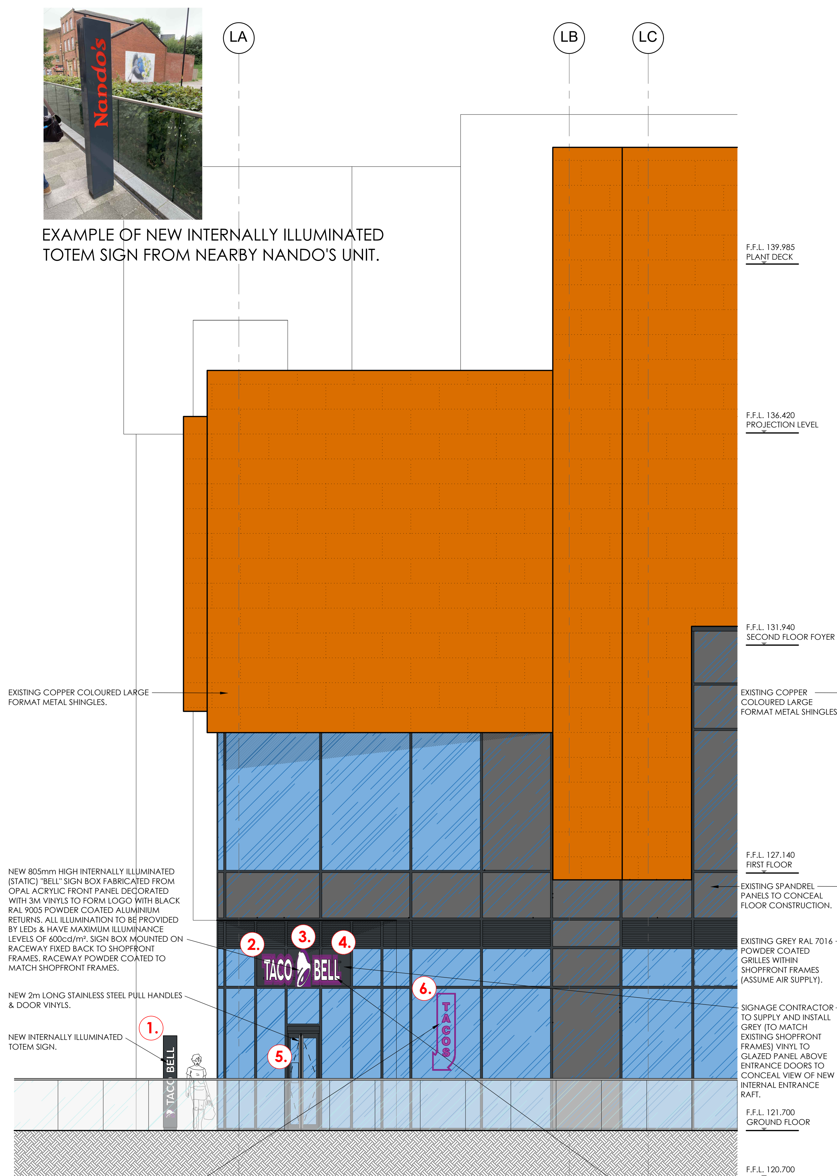
proposed West facing elevation scale - 1:50 @ A1 / 1:100 @ A3
