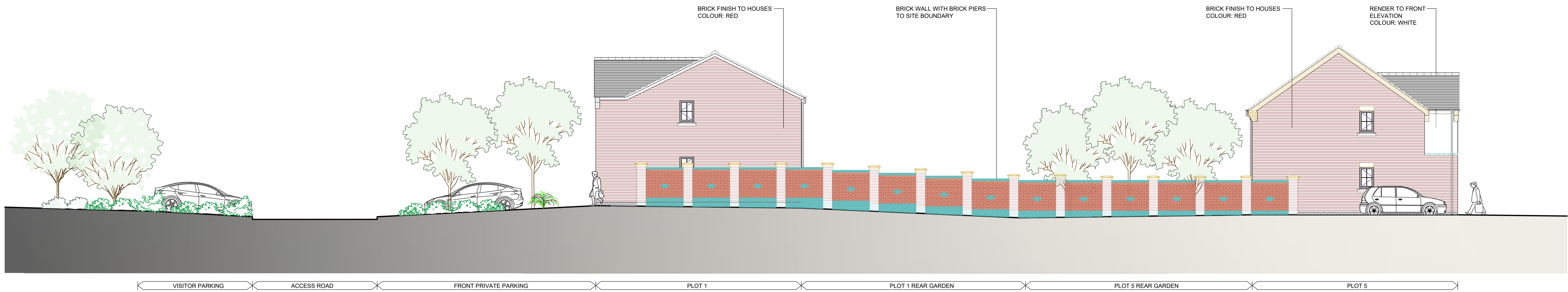
PROPOSED WESTERN ELEVATION SCALE : 1:100
