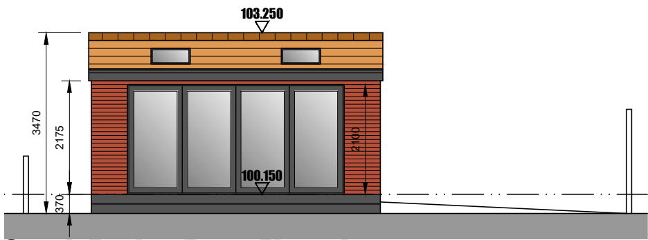
South Facing Front Elevation
