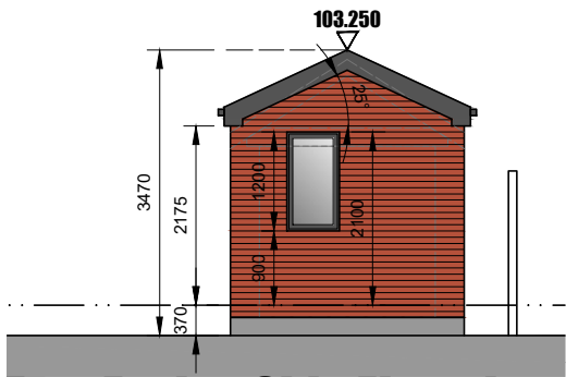
East Facing Side Elevation
