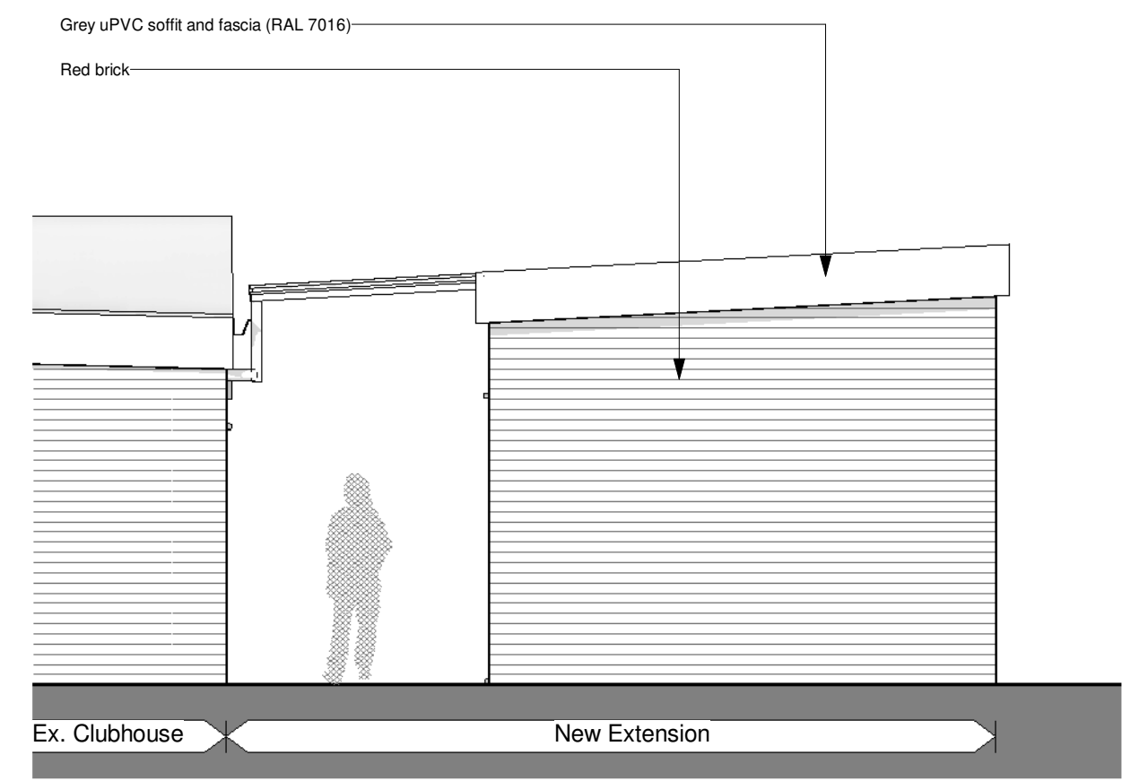
West Elevation 1 : 50
