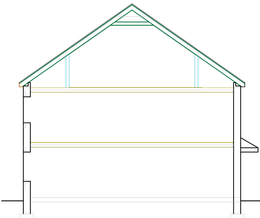
PROPOSED SKETCH SECTION
