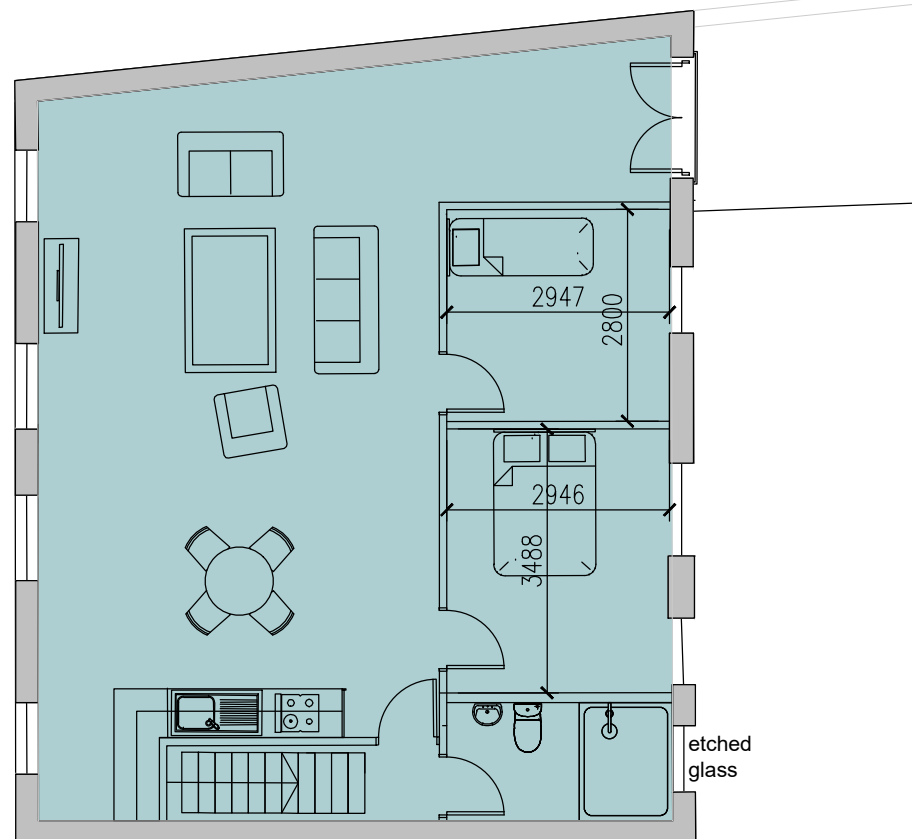
FIRST FLOOR PLAN - FLAT 4 Proposed GIA: 83 sqm
