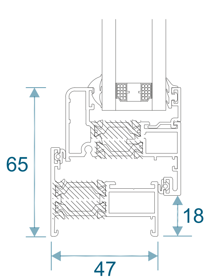
Opening Vents With Outer Frame
