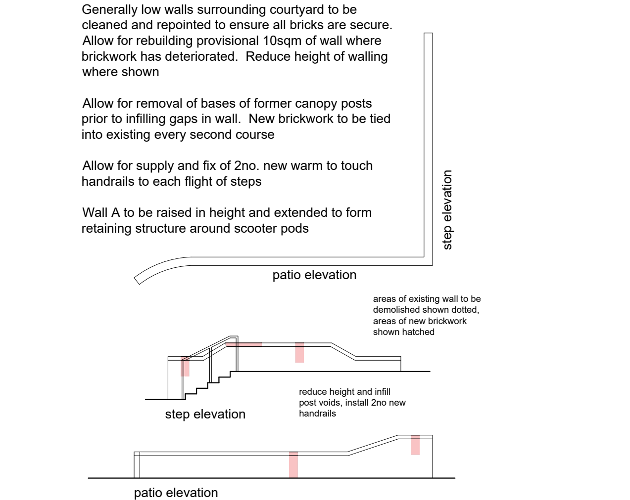
Proposed Plan and Elevation of Wall D Proposed Plan and Elevation of Wall E
