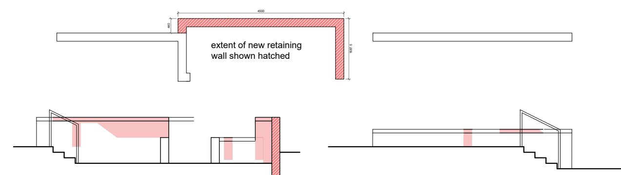
Proposed Plan and Elevation of Wall A Proposed Plan and Elevation of Wall C
