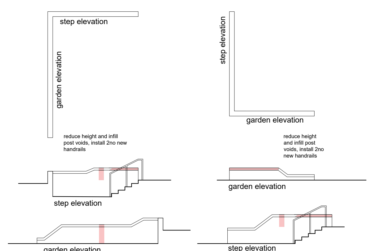
Proposed Plan and Elevation of Wall D Proposed Plan and Elevation of Wall E
