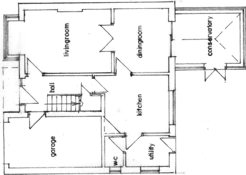
G.F. PLAN (EXISTING)
