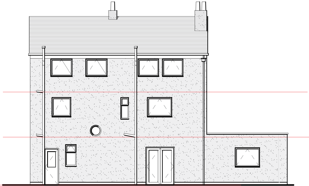
Rear Elevation
