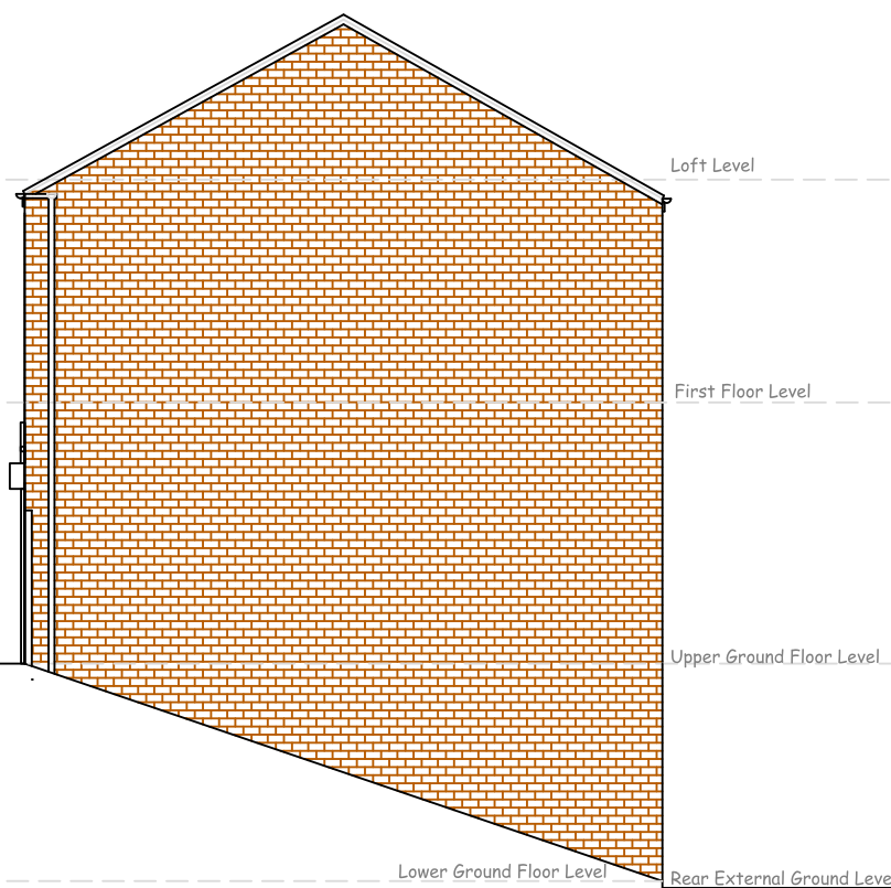
RH SIDE ELEVATION – AS EXISTING 1:100
