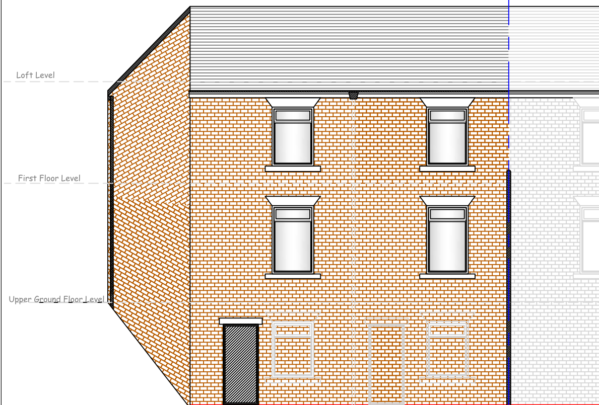
REAR ELEVATION – AS EXISTING 1:100
