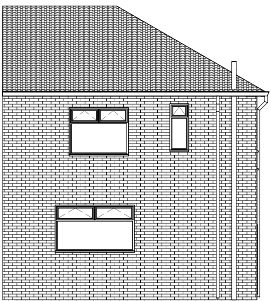
Existing Rear 1 : 100
