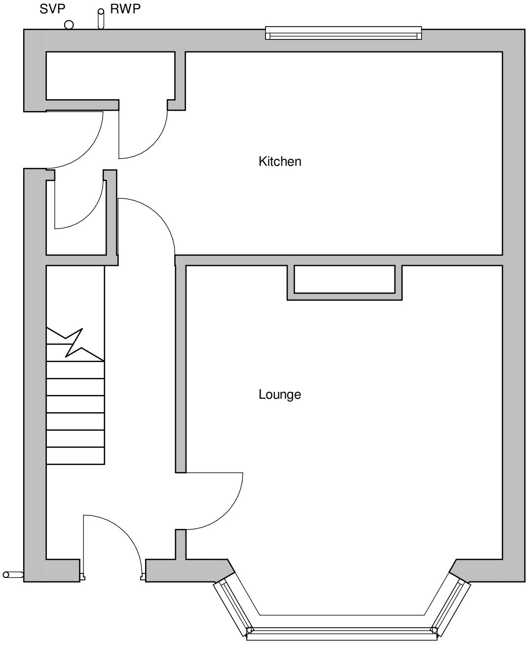
Existing Ground Floor 1 : 50
