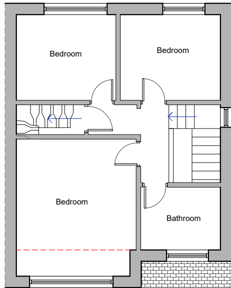
Existing First Floor Plan 1:100 @ A3
