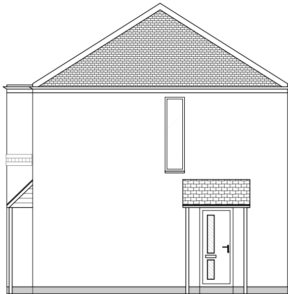
Existing Side Elevation 1:100 @ A3
