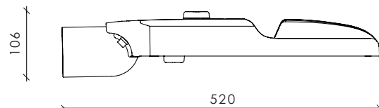
Dimensions with 2 Zhaga connectors
