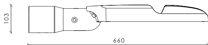
Dimensions with adjustable console \pm 90^\circ , 76 mm
