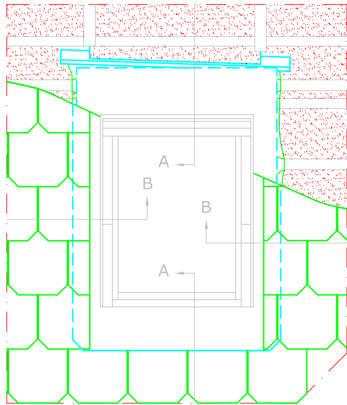
TYPICAL ELEVATION
