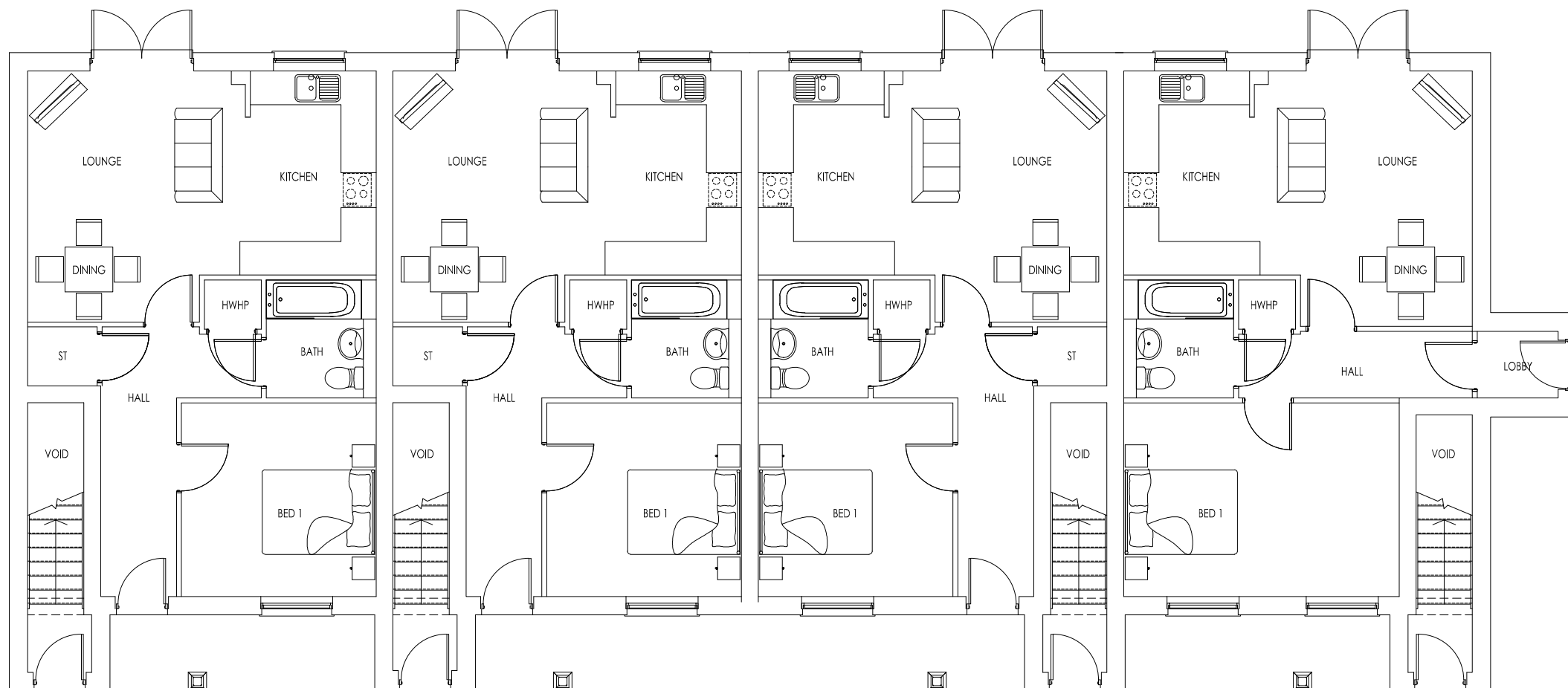
Ground Floor
