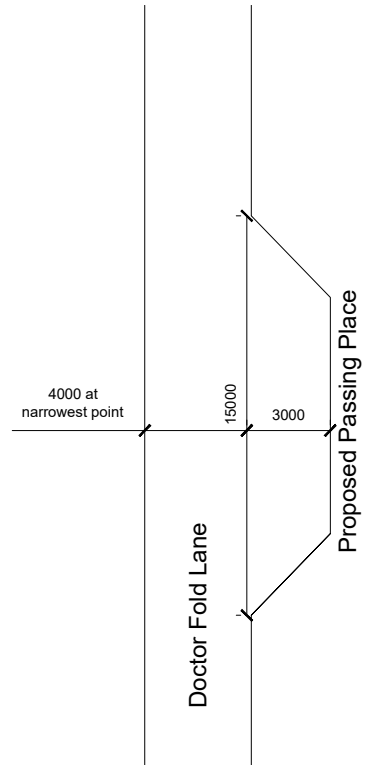
TYPICAL PASSING PLACE DETAIL
