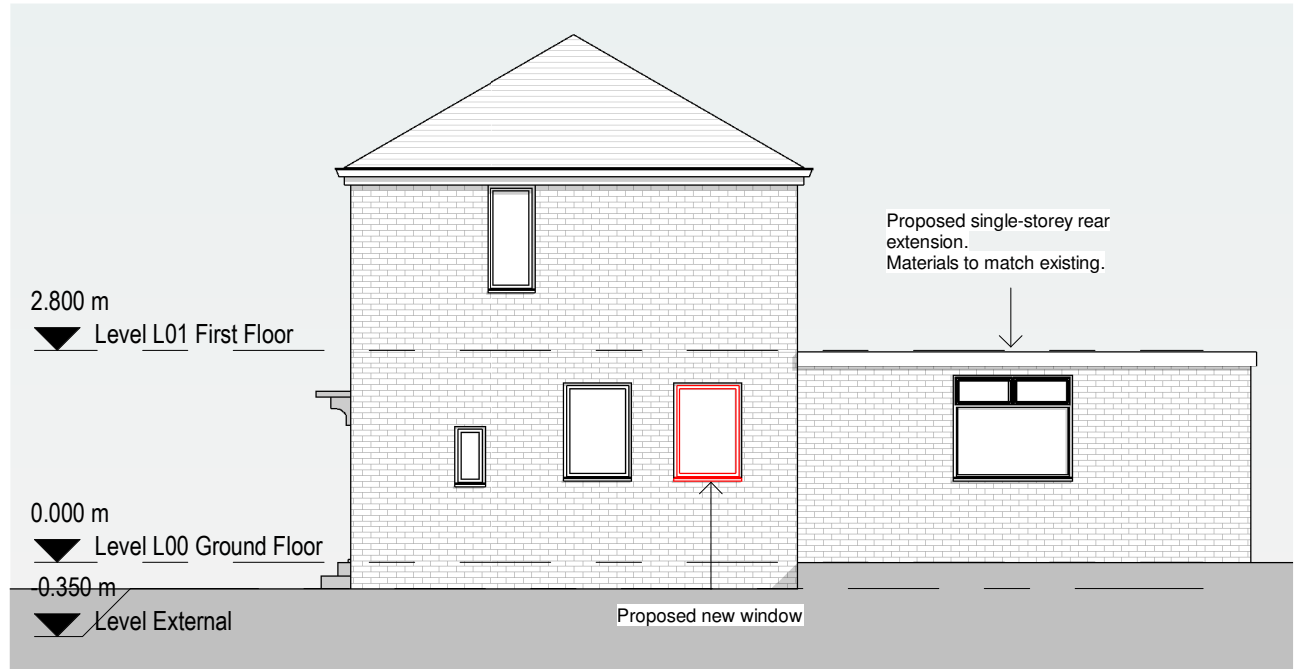
2 Proposed West Elevation 1 : 100
