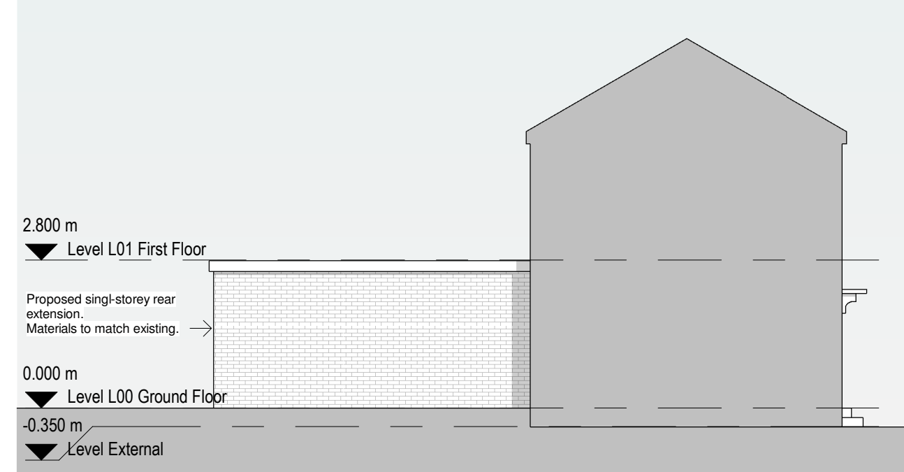
4 Proposed East Elevation 1 : 100
