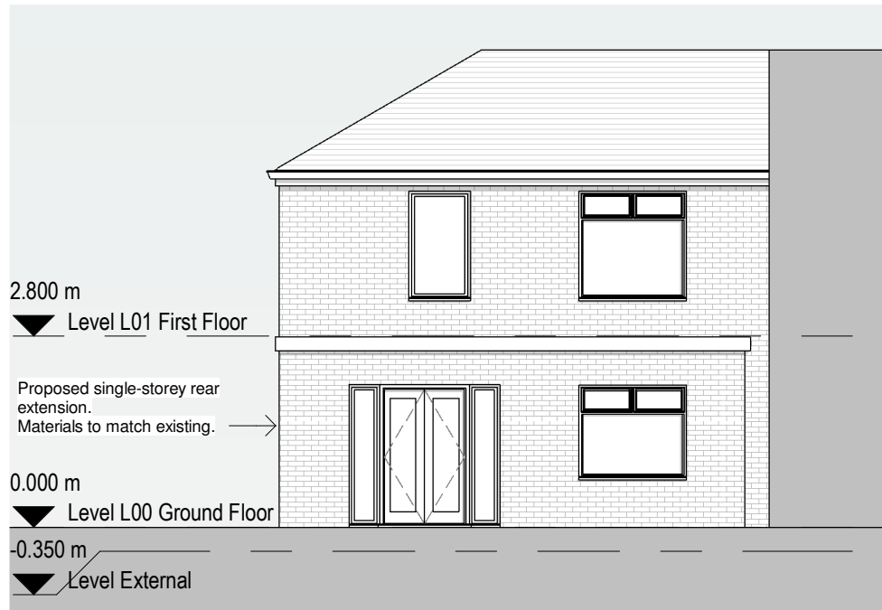
3 Proposed South Elevation 1 : 100
