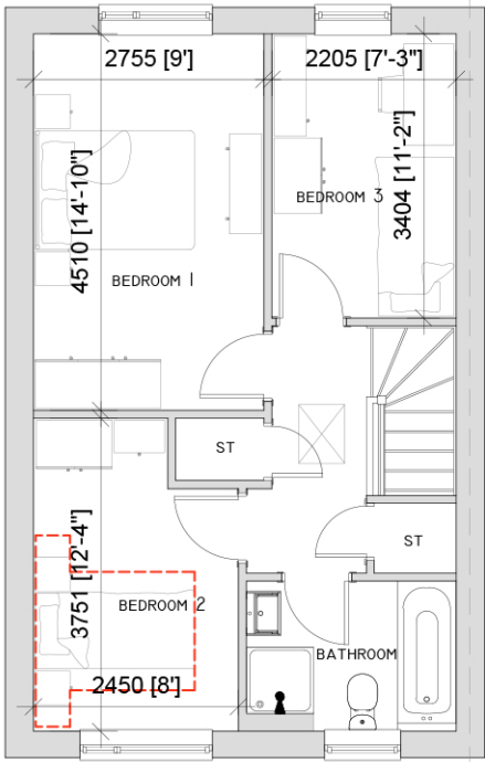
FIRST FLOOR - 42.22m²/454sqft
