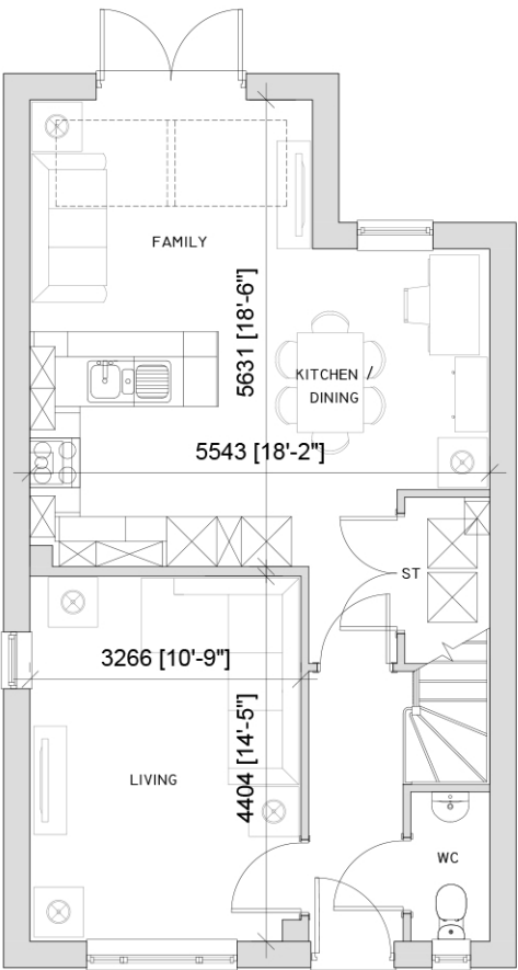
GROUND FLOOR - 52.44m 2 /564sqft
