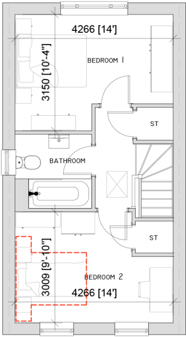
FIRST FLOOR - 35.64m²/383.5sqft
