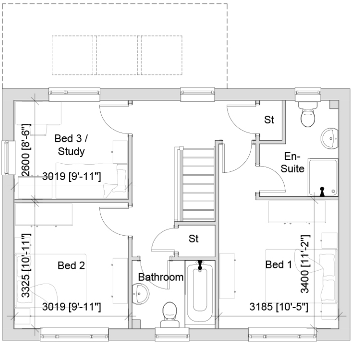
FIRST FLOOR - 51.73m 2 /556sqft
