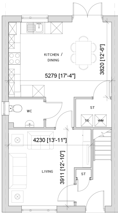
GROUND FLOOR - 49.62m 2 /532sqft
