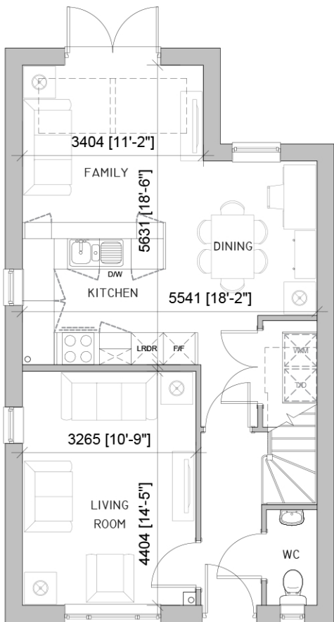
GROUND FLOOR - 52.43m 2 /564sqft
