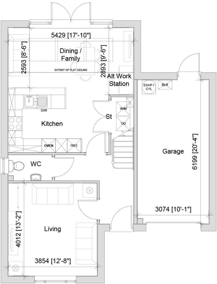
GROUND FLOOR - 54.63m 2 /588sqft
