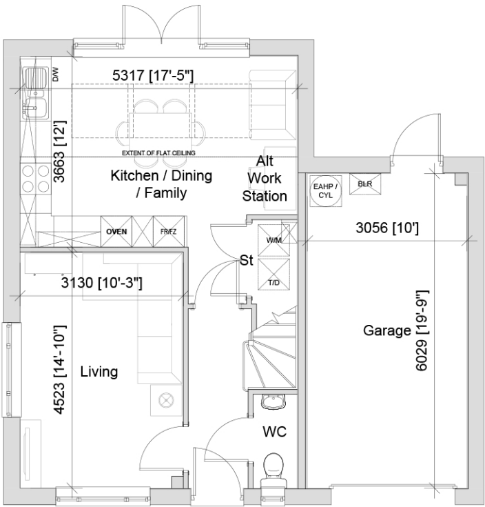
GROUND FLOOR - 44.02m 2 /474sqft
