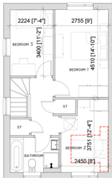
FIRST FLOOR - 42.38m 2 /454sqft
