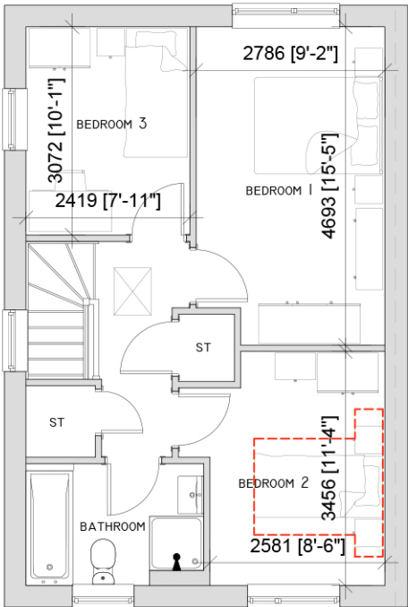
FIRST FLOOR - 43.66m 2 /469.5sqft
