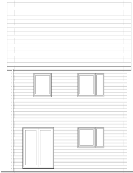
REAR ELEVATION
