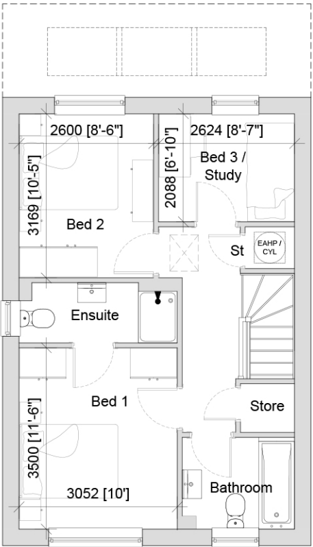
FIRST FLOOR - 42.62m 2 /459sqft
