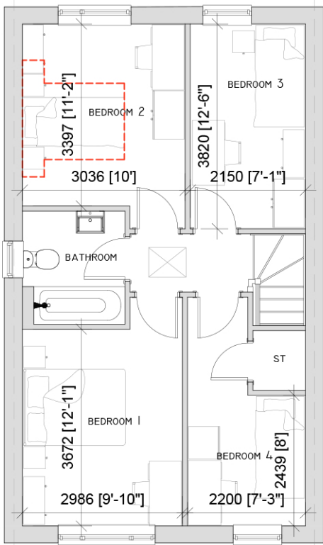
FIRST FLOOR - 49.62m 2 /532sqft
