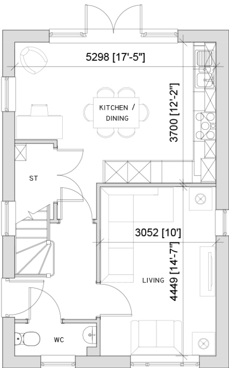
GROUND FLOOR - 43.66m 2 /469.5sqft
