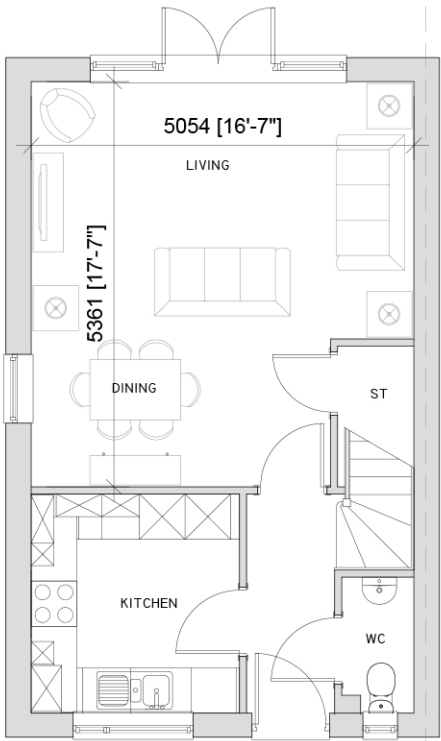
GROUND FLOOR - 42.22m²/454sqft
