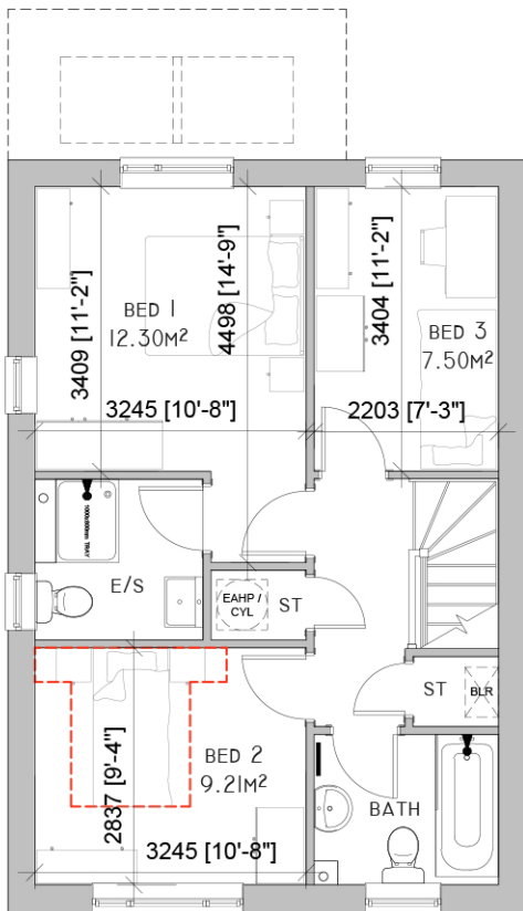
FIRST FLOOR - 46.30m 2 /498sqft
