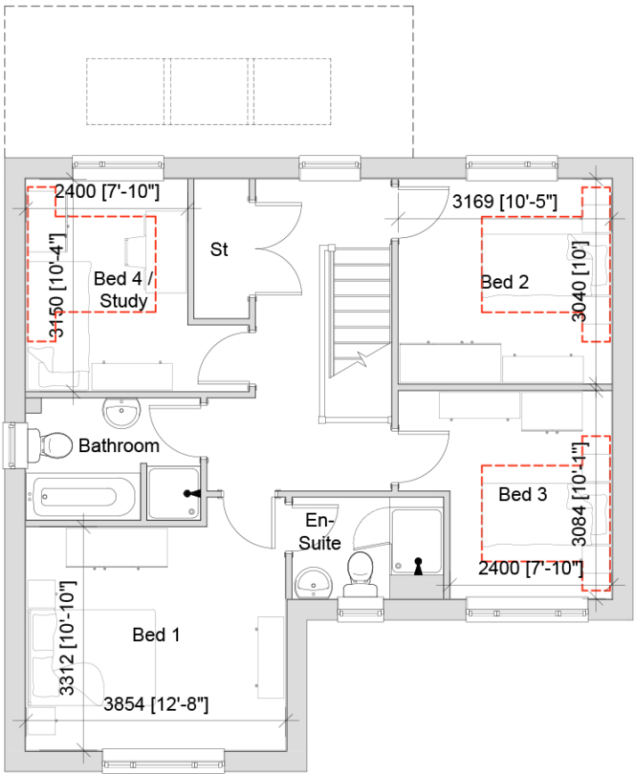
FIRST FLOOR - 62.67m 2 /675sqft
