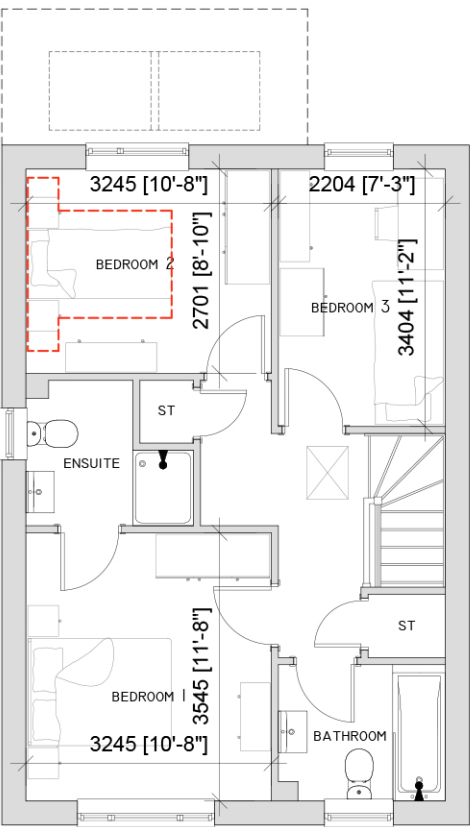
FIRST FLOOR - 46.27m 2 /498sqft
