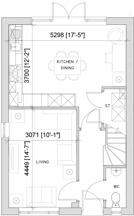
GROUND FLOOR - 43.505m 2 /468sqft
