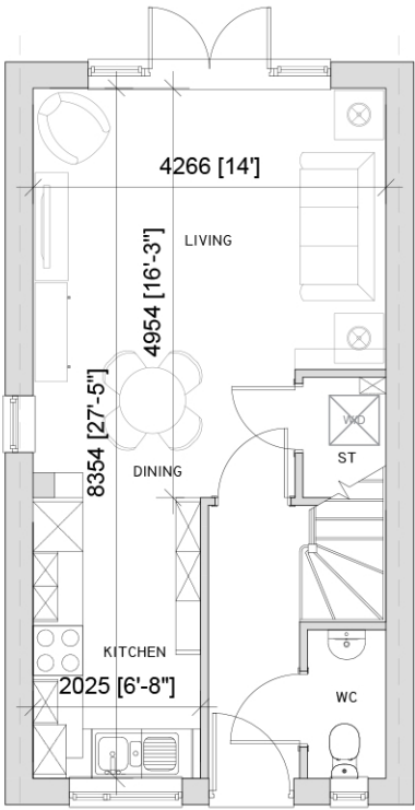
GROUND FLOOR - 35.64m²/383.5sqft
