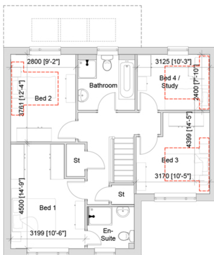
FIRST FLOOR - 63.96m 2 /688sqft
