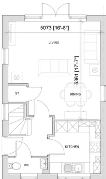
GROUND FLOOR - 42.38m 2 /454sqft
