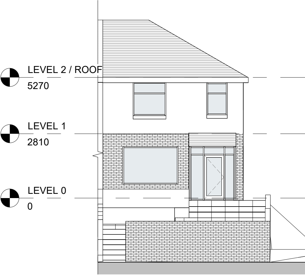
1 Front - Existing 1 : 100
