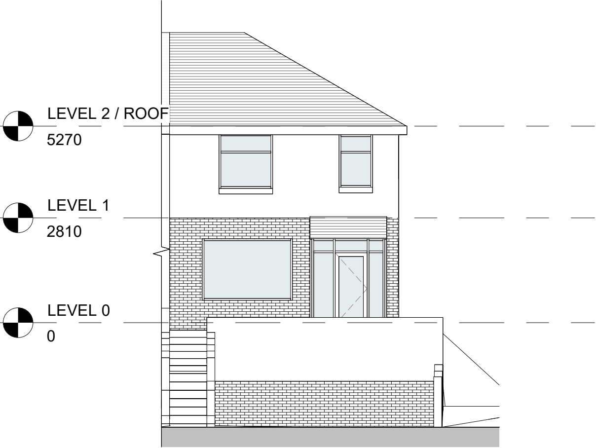
2 Front - Proposed 1 : 100
