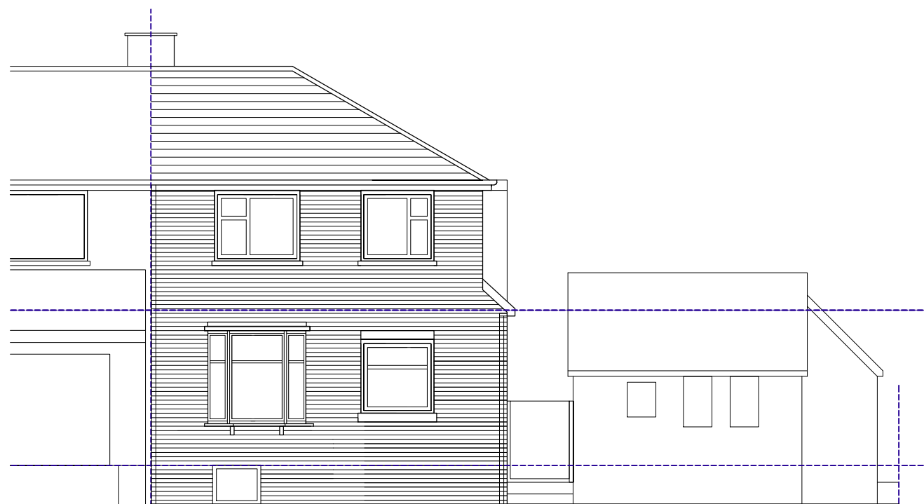
REAR ELEVATION
