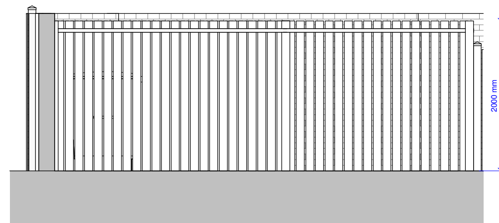
5 Proposed Side Elevation _Bin Store 1 : 50
