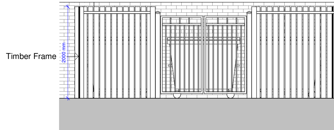
3 Proposed Front Elevation _Bin Store 1 : 50
