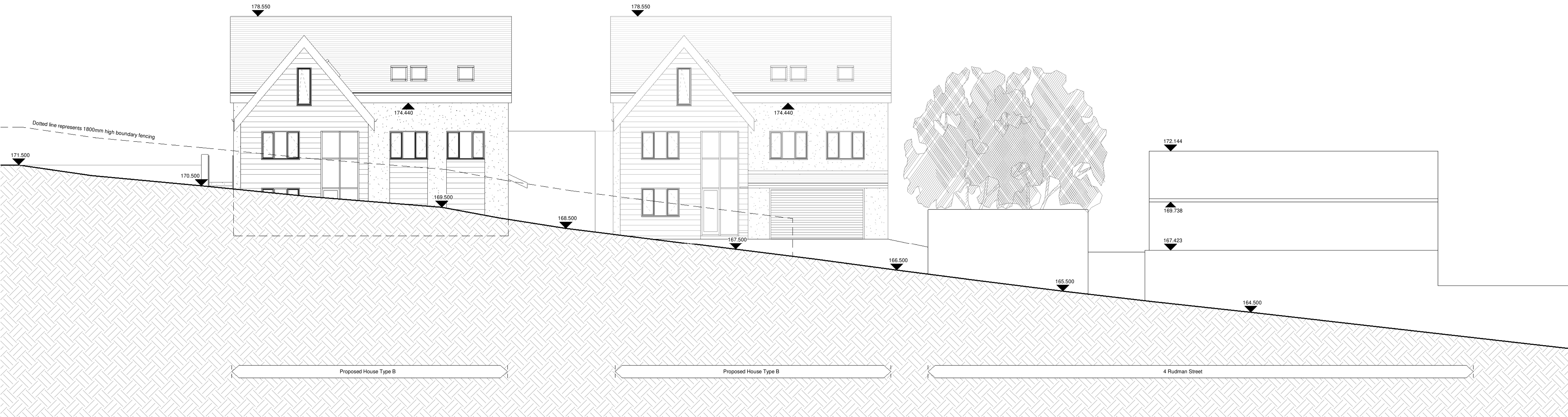
Proposed Streetscene Elevation 1 : 100
