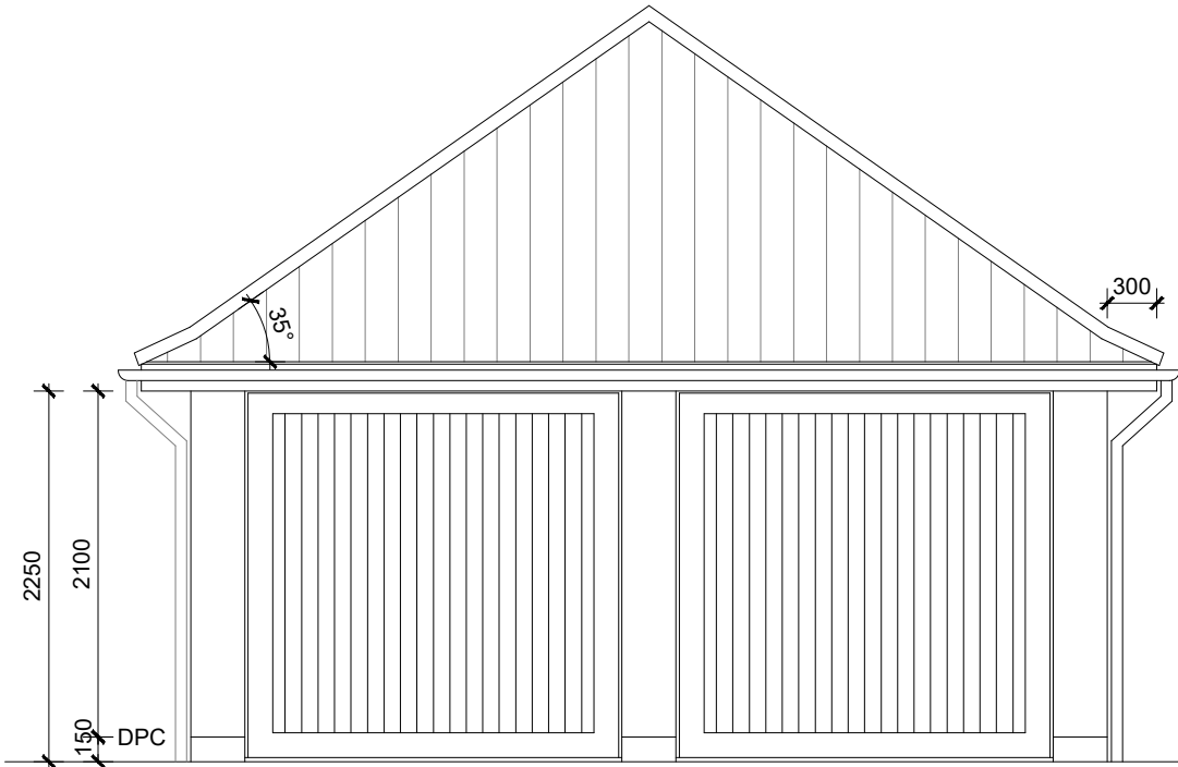
FRONT ELEVATION
