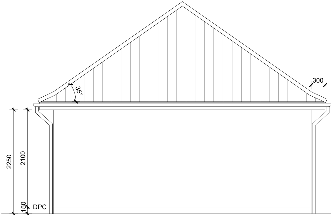
REAR ELEVATION
