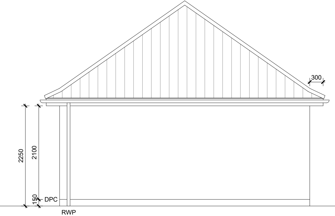
SIDE ELEVATION
