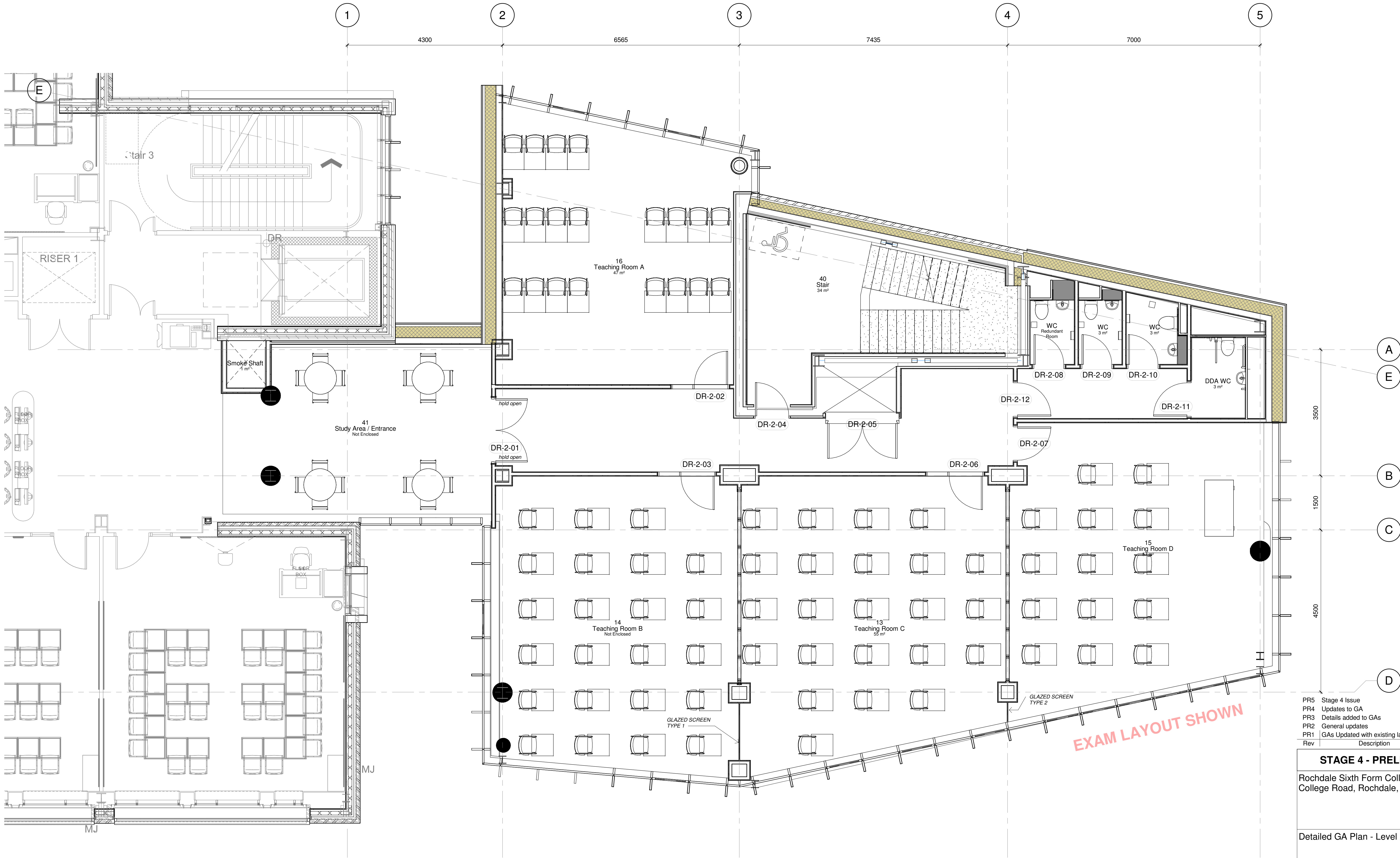
Detailed GA Plan - Level 2 1 : 50
