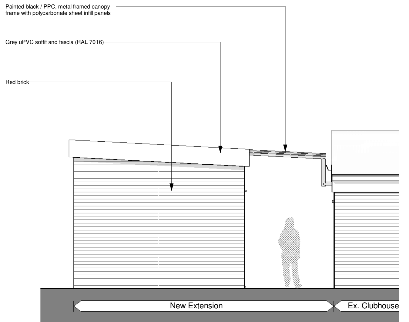
East Elevation 1 : 50
