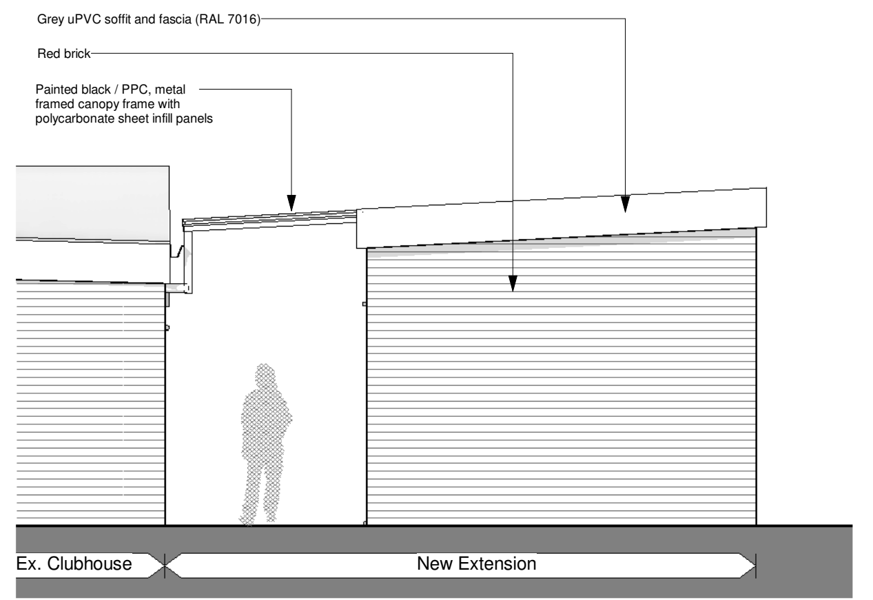
West Elevation 1 : 50
