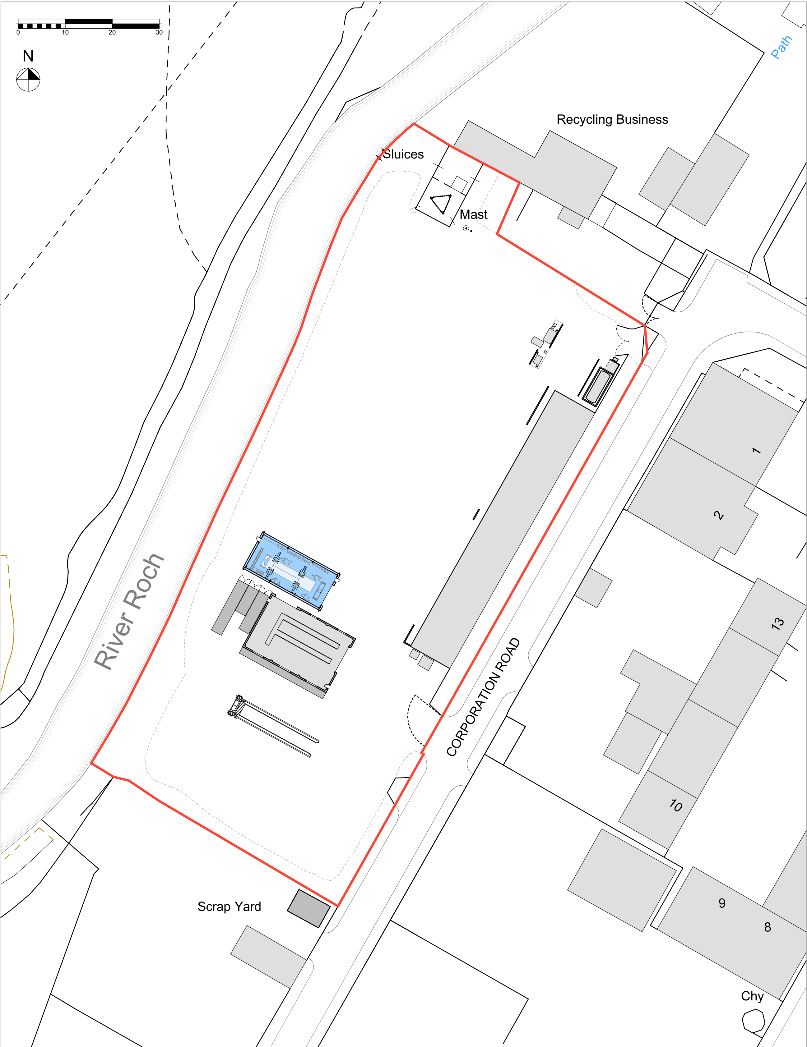
Block Plan - As Proposed Scale 1:500
