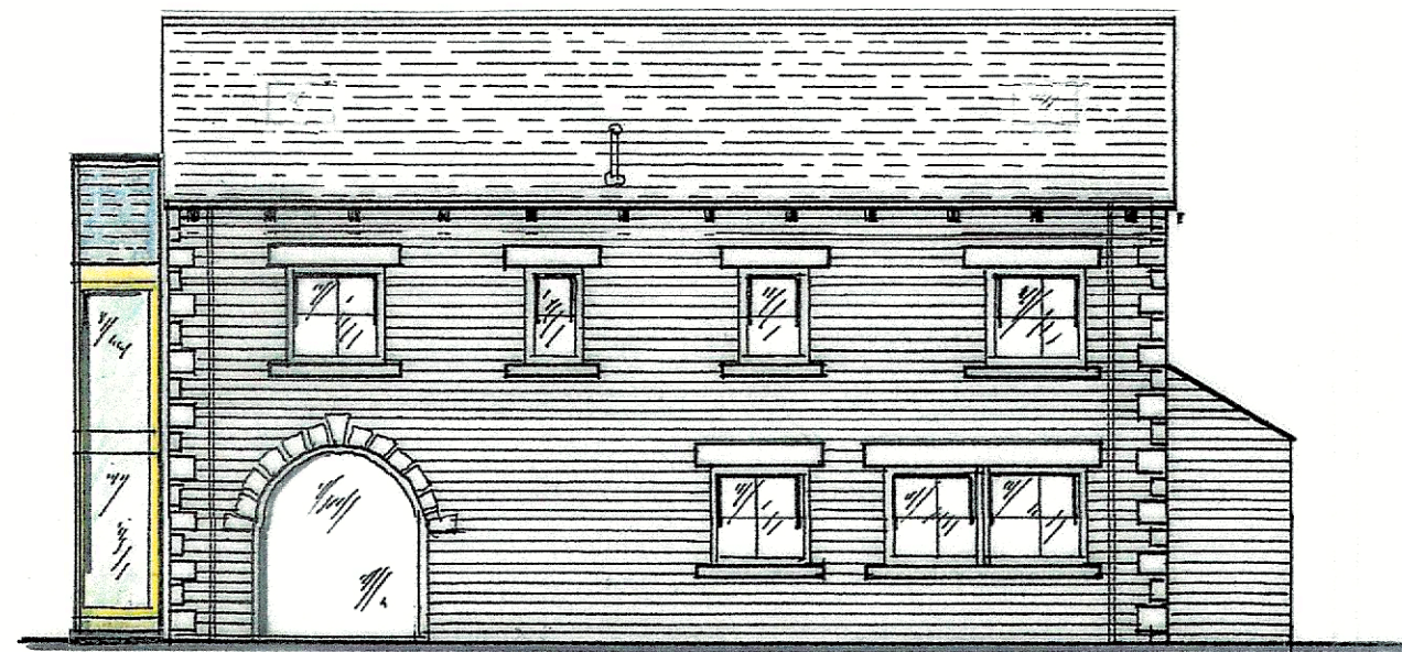
SOUTH ELEVATION.
