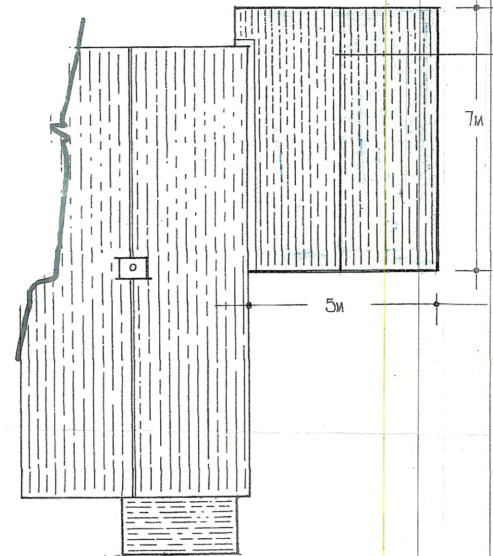
ROOF PLAN 1:200
