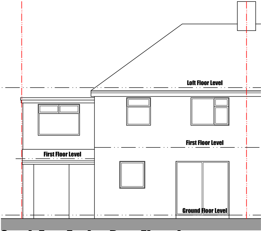
South East Facing Rear Elevation
