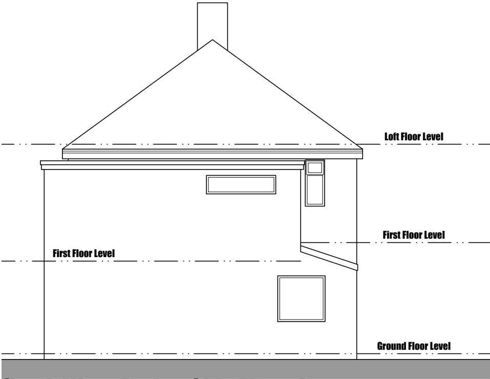
South West Facing Side Elevation
