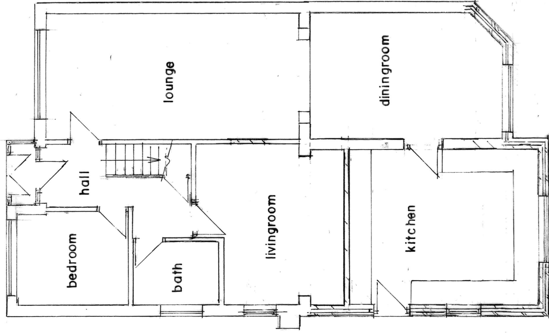
GROUND FLOOR PLAN (PROPOSED)
