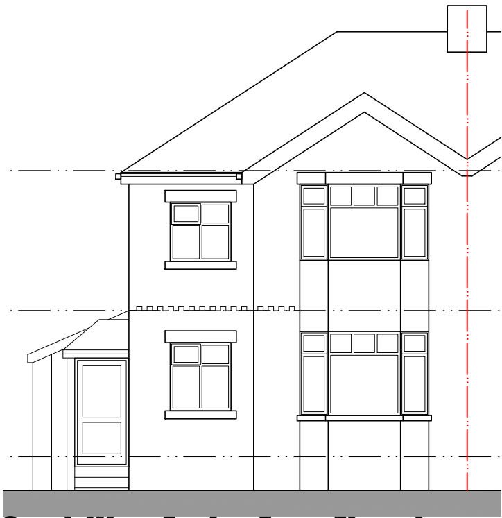
South West Facing Front Elevation
