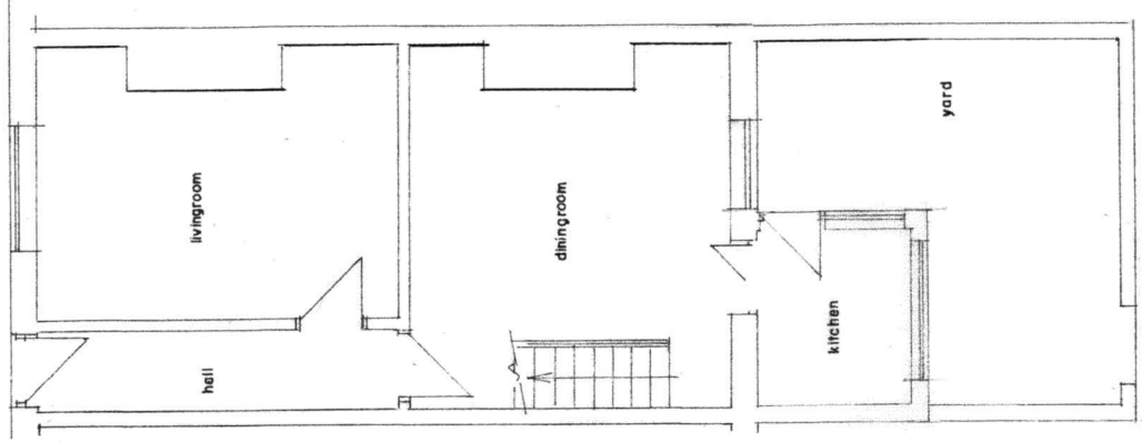
G.F. PLAN (EXISTING)
