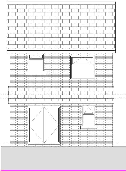
PROPOSED HOUSE 1 REAR ELEVATION 1:100 @ A3
