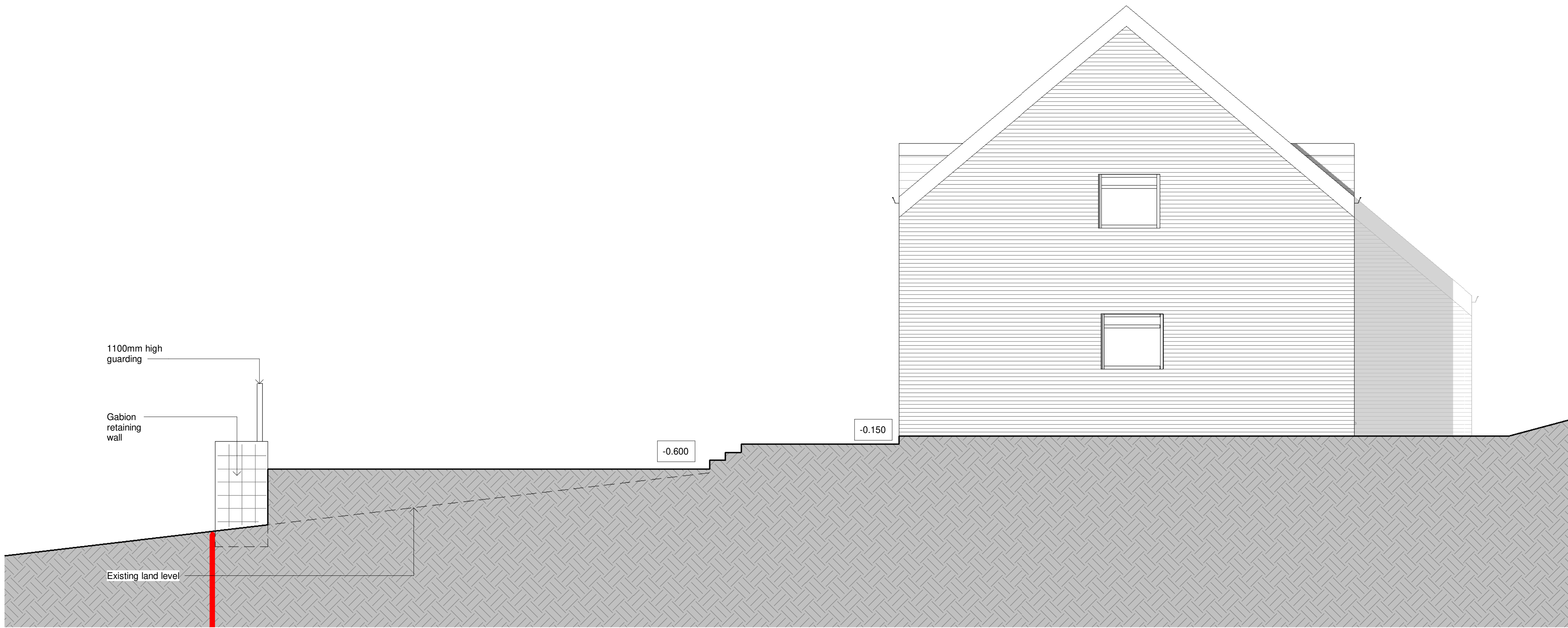
Proposed Site Section 1 : 50
