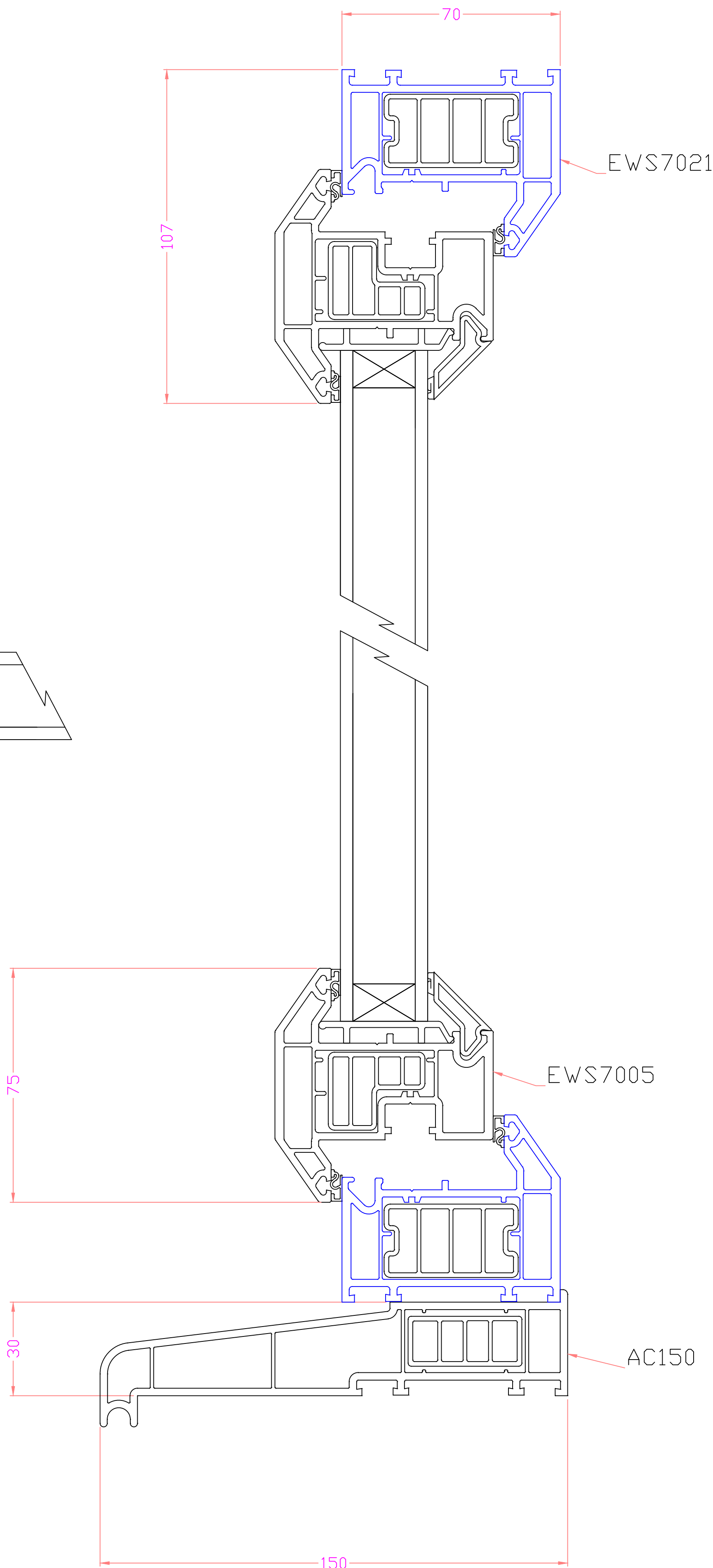
Section Y-Y
