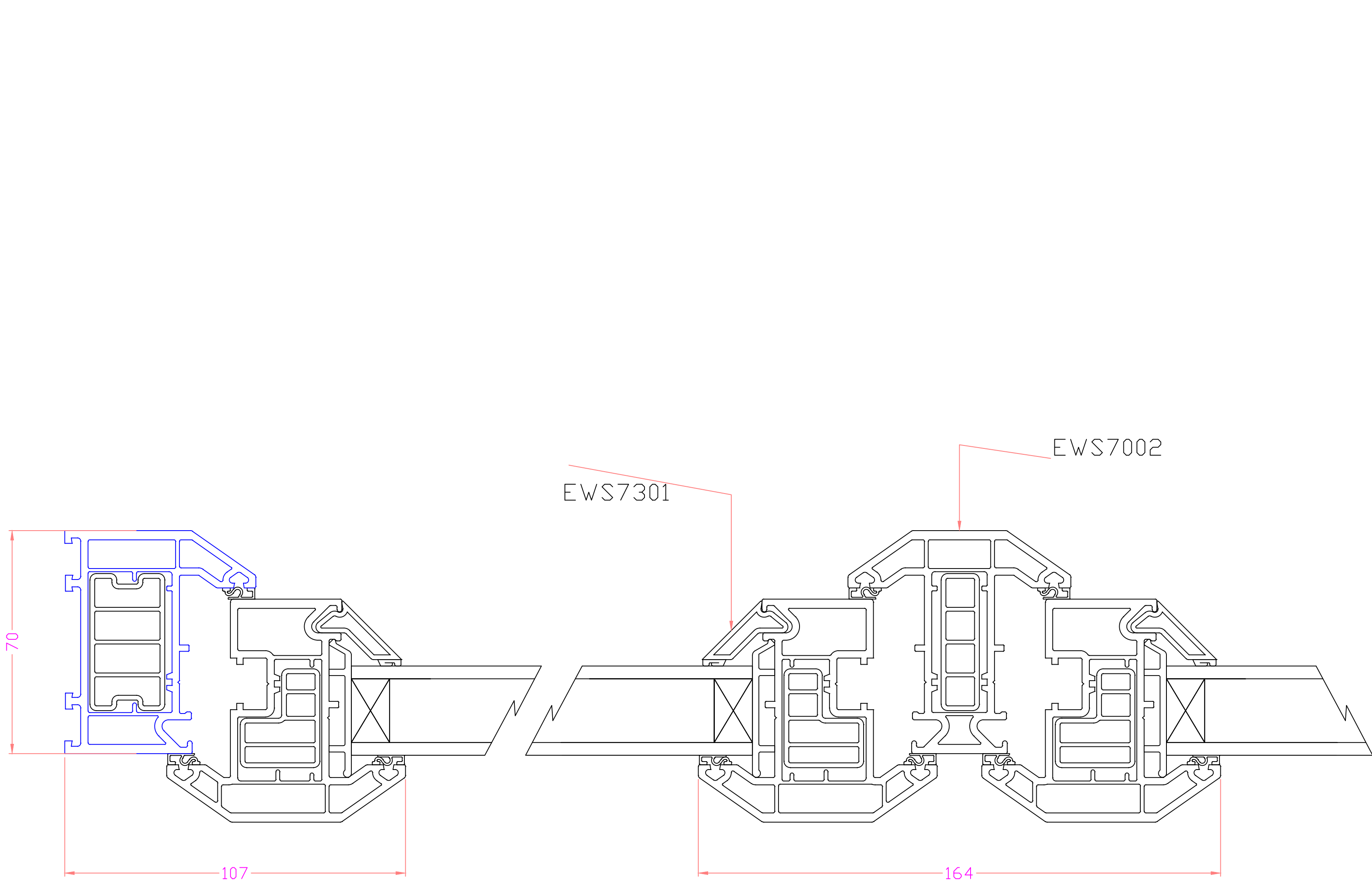
Section X-X
