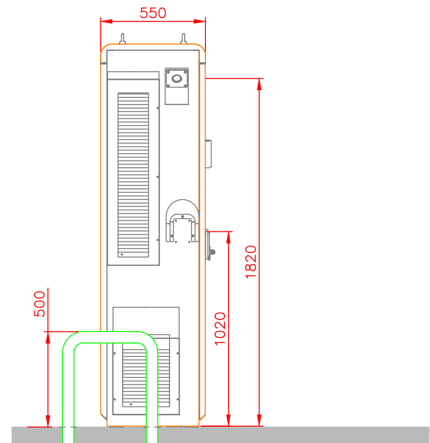
BYD CHARGING POINT SIDE ELEVATION
