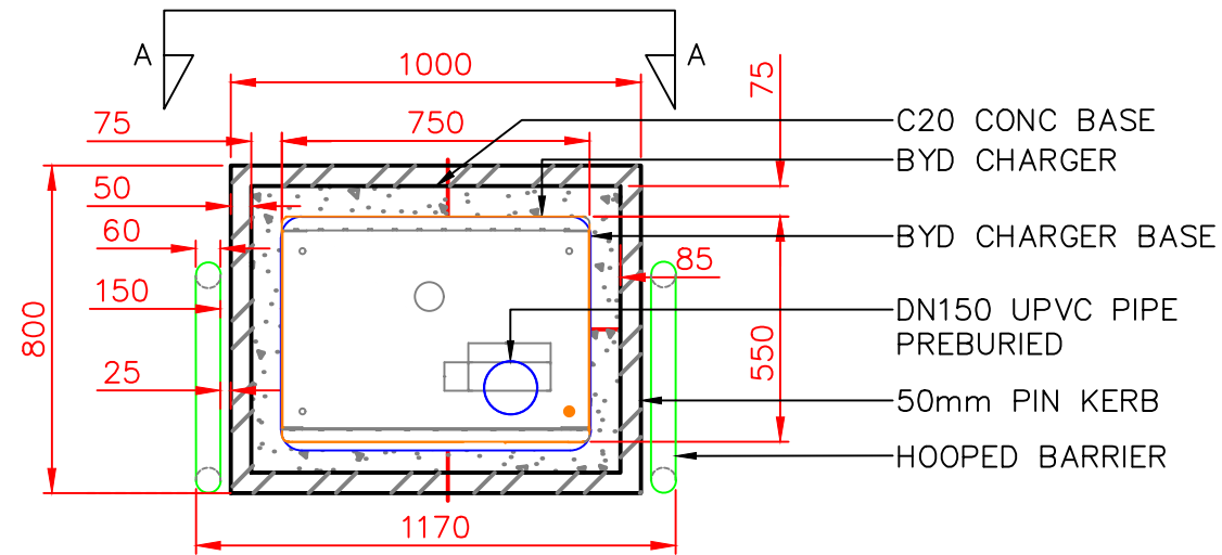
BYD CHARGING POINT PLAN DETAIL
