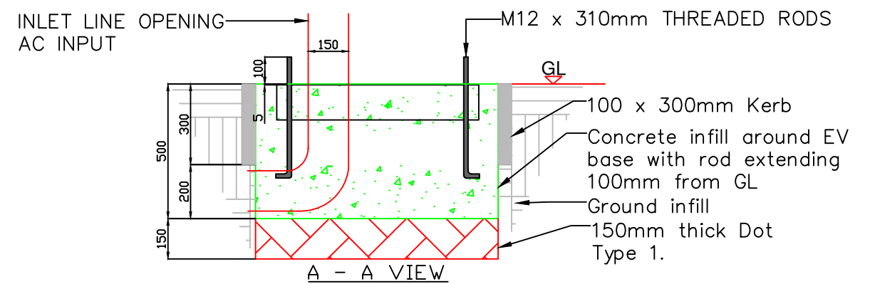
BYD CHARGING POINT FOUNDATION SECTION
