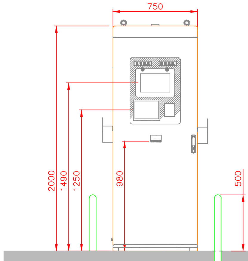
BYD CHARGING POINT FRONT ELEVATION
