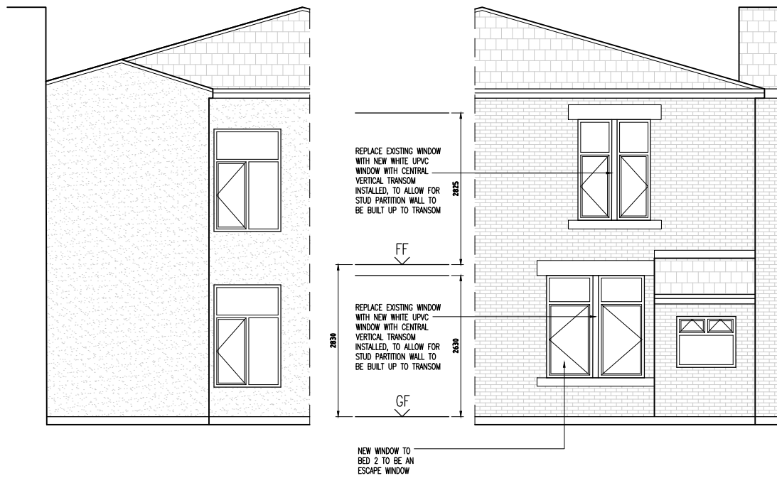
PROPOSED REAR ELEVATION 1:100 @ A3
