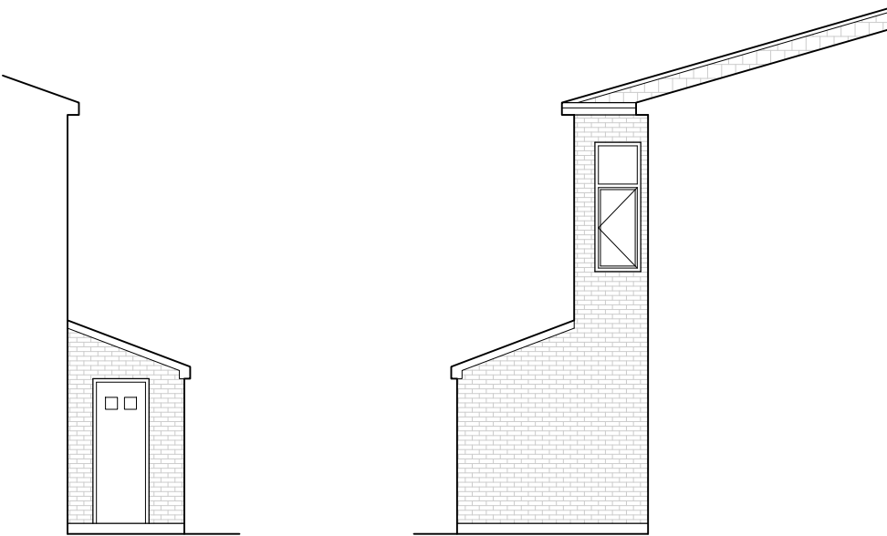
PROPOSED SIDE FRONT ELEVATION 1:100 @ A3
