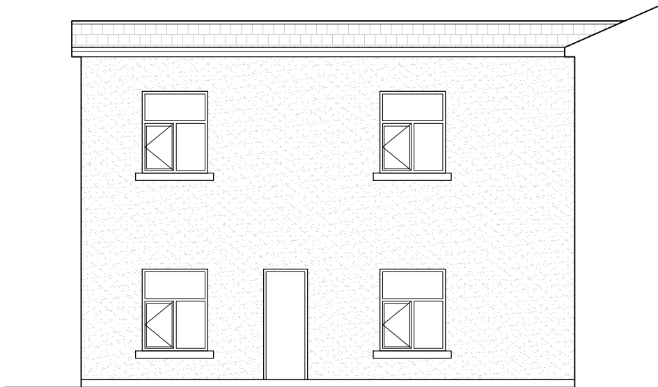
PROPOSED REAR/SIDE ELEVATION 1:100 @ A3
