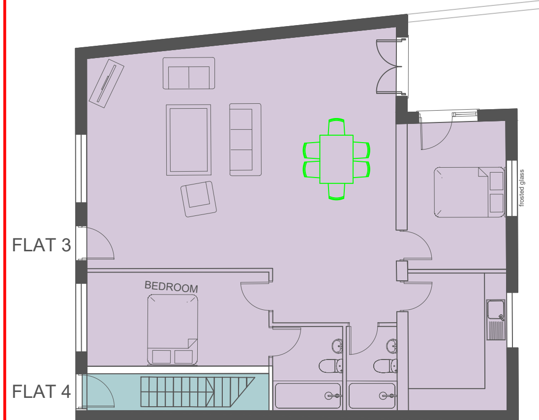
GROUND FLOOR PLAN - FLAT 3 Proposed GIA: 101 sqm
