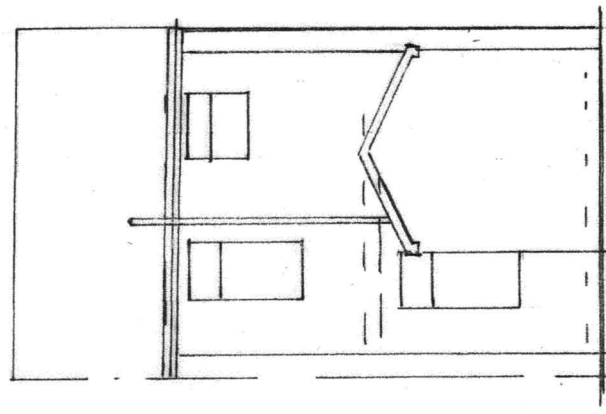
REAR ELEVATION (EXISTING)
