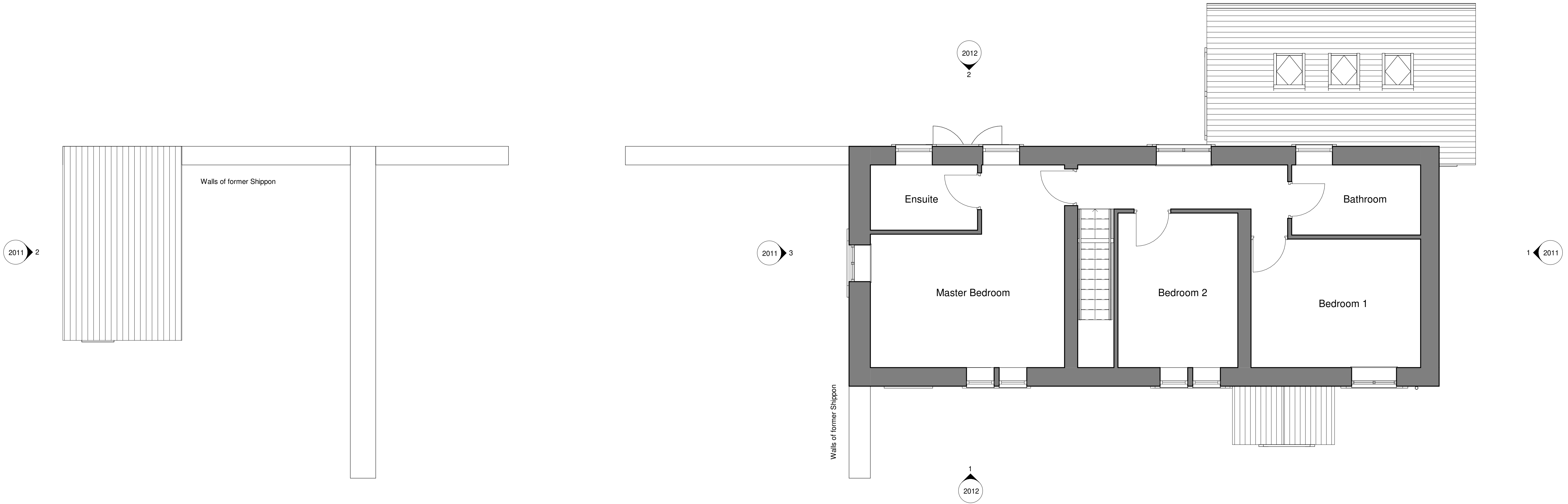
2 | Ex Level 1
