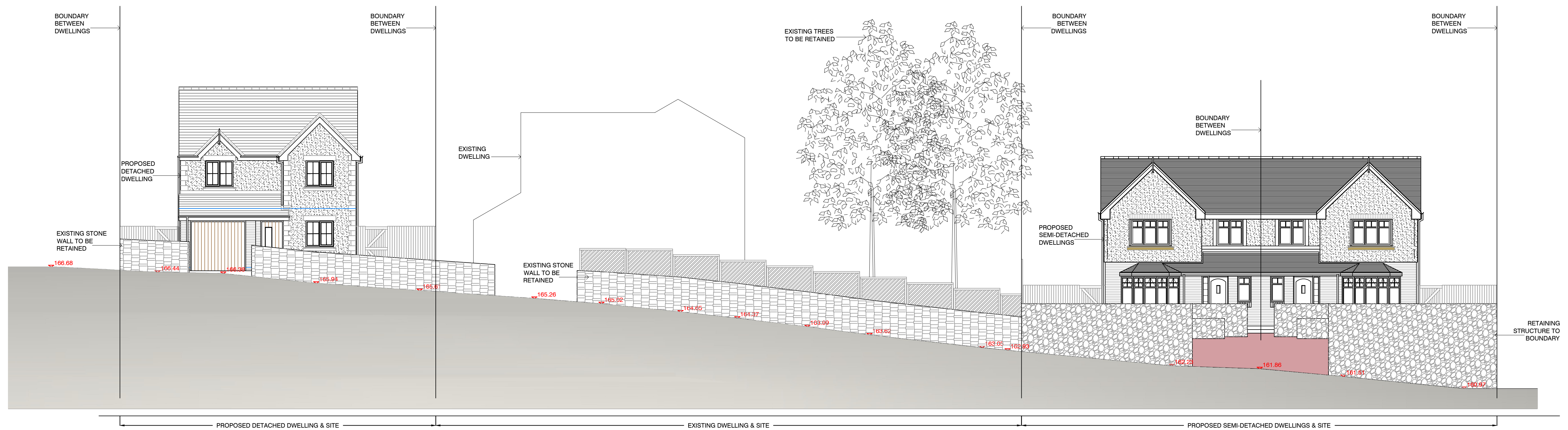
STREET SCENE ELEVATION 1:100
