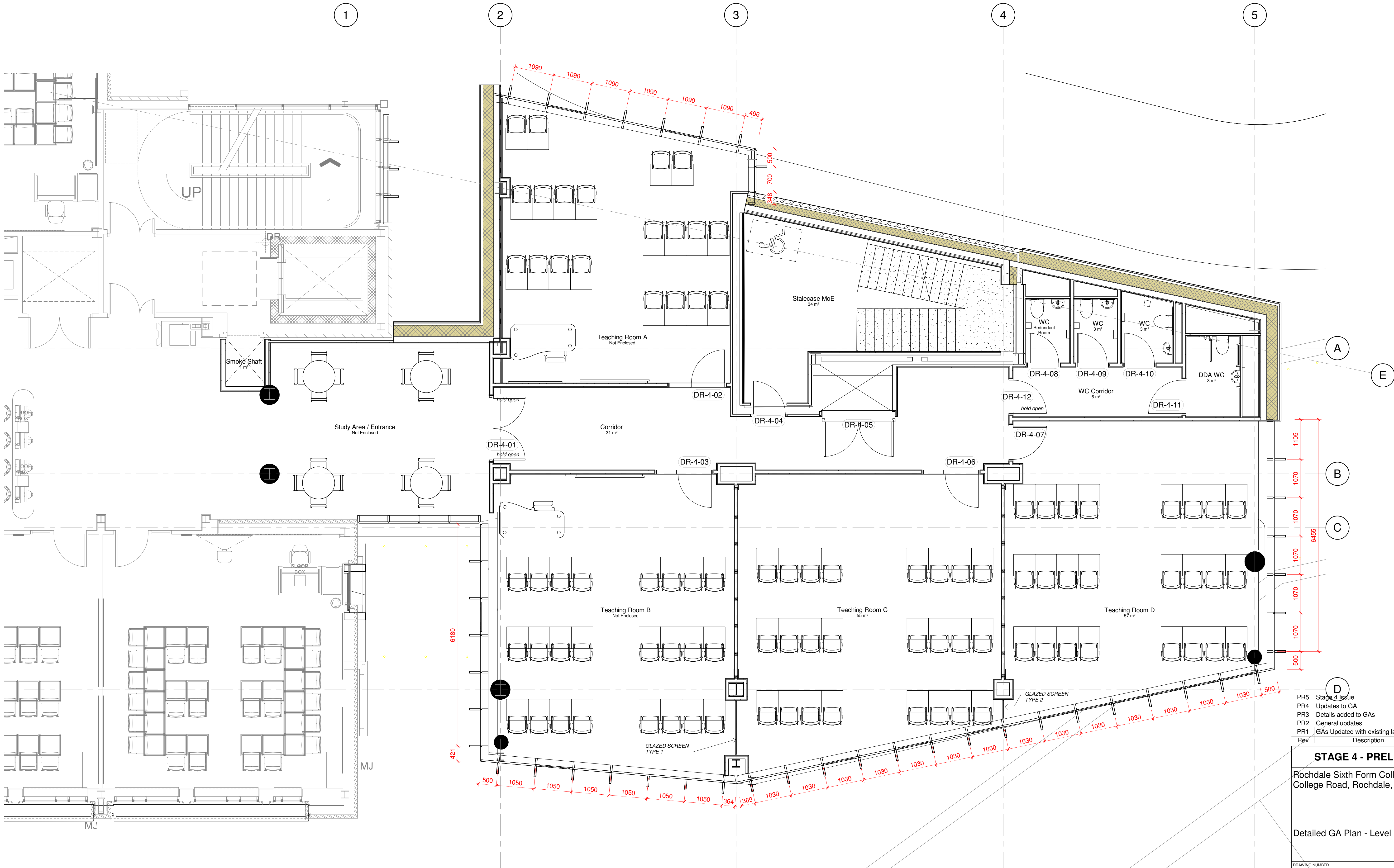
Detailed GA Plan - Level 4 1 : 50
