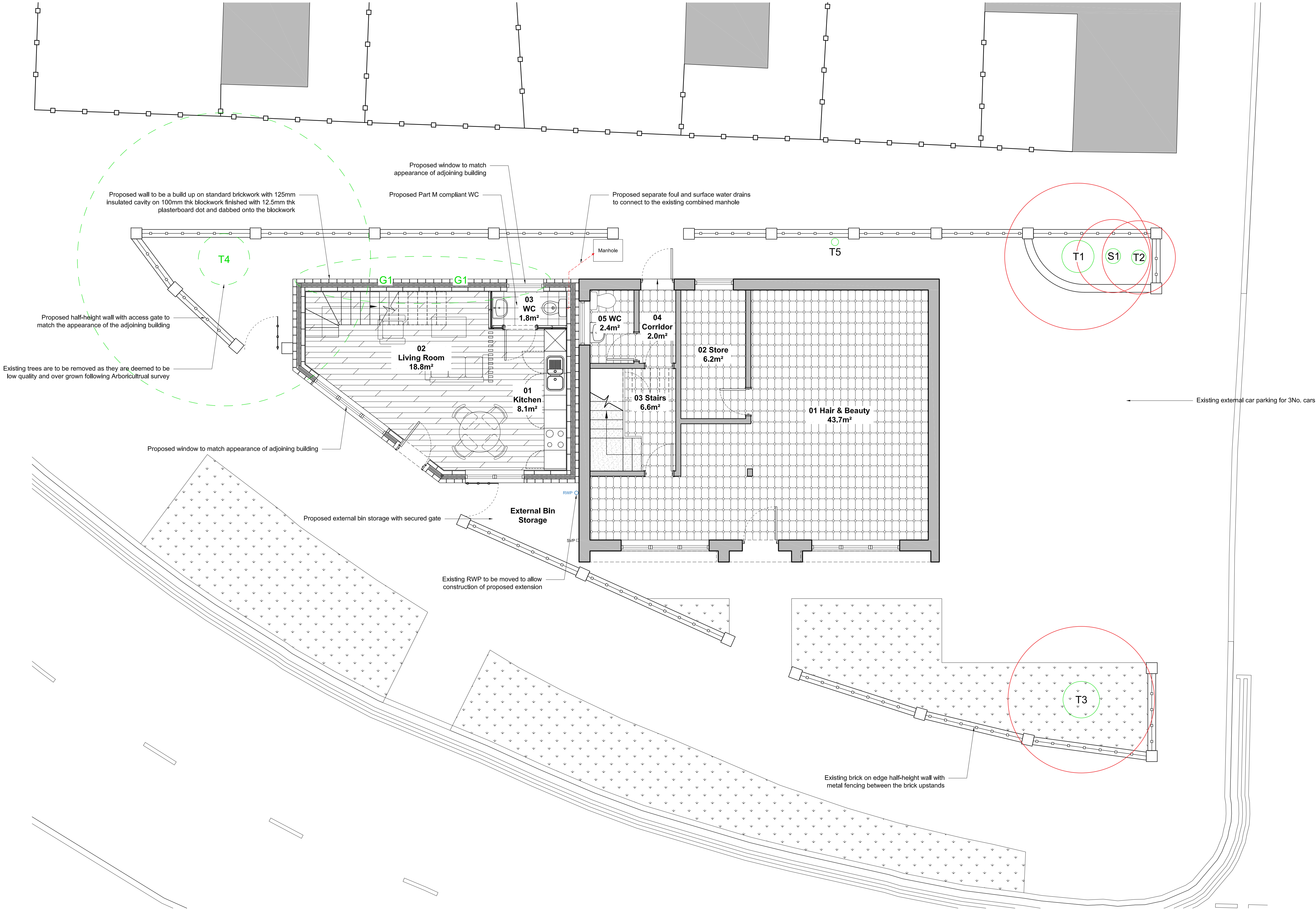
01 PROPOSED GA PLAN Scale 1:50 @ A1
