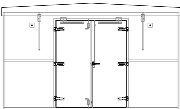
ELEVATION @ `B`
