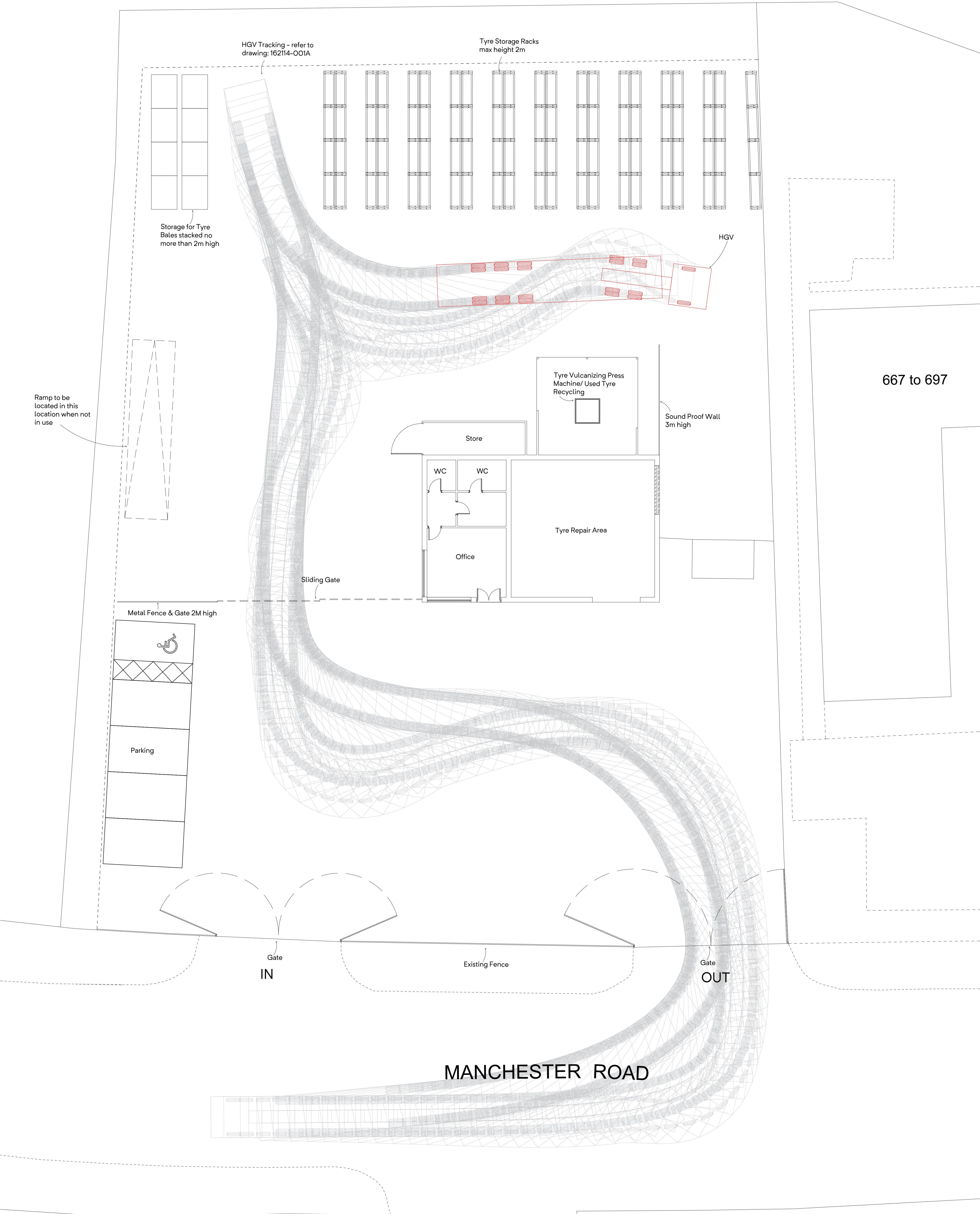
SITE PLAN (PROPOSED)
